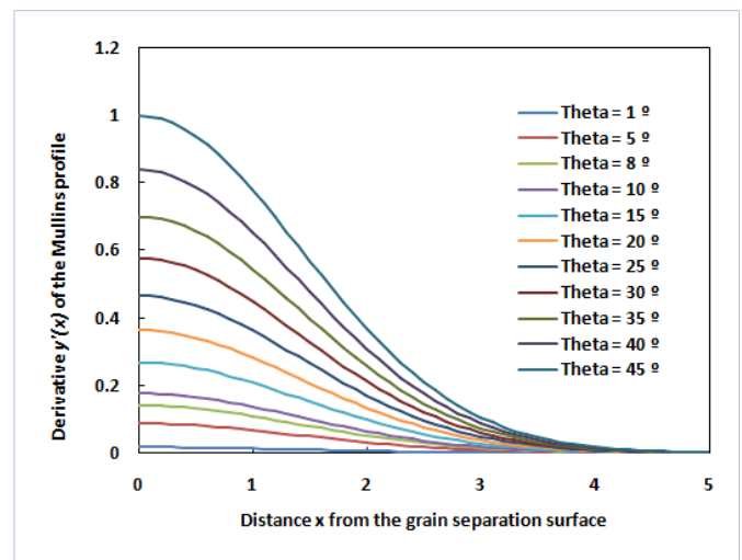
Figure 6: Evolution of the derivative y'(x) of the grain groove profile of Mullins approximation as a function of the distance x from the grain separation surface for various groove angles \theta .
