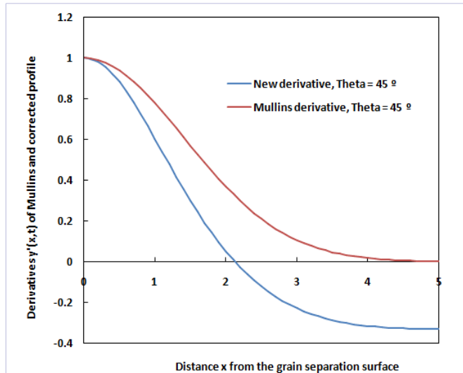
Figure 11: Evolution of the derivative y'(x) of the grain groove profile for Mullins approximation and the new proposed solution as a function of the distance x from the grain separation surface for \theta = 45^\circ
