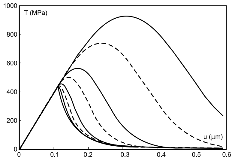
Fig. 28. The responses of the model by Cangémi et al. for various rates of controlled displacement: (—): \dot{u} = 10^{-4}, 0.01, 0.1, 1, 10 \mu\text{m/s} and (---): \dot{u} = 0.04, 0.4, 4 \mu\text{m/s} .
