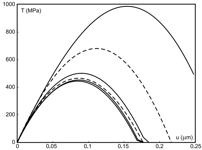
Fig. 27. The responses of the Allix–Ladevèze model for various rates of controlled displacement: (—): \dot{u} = 10^{-3}, 0.1, 1, 10 \mu\text{m/s} and (---): \dot{u} = 0.4, 4 \mu\text{m/s} .
