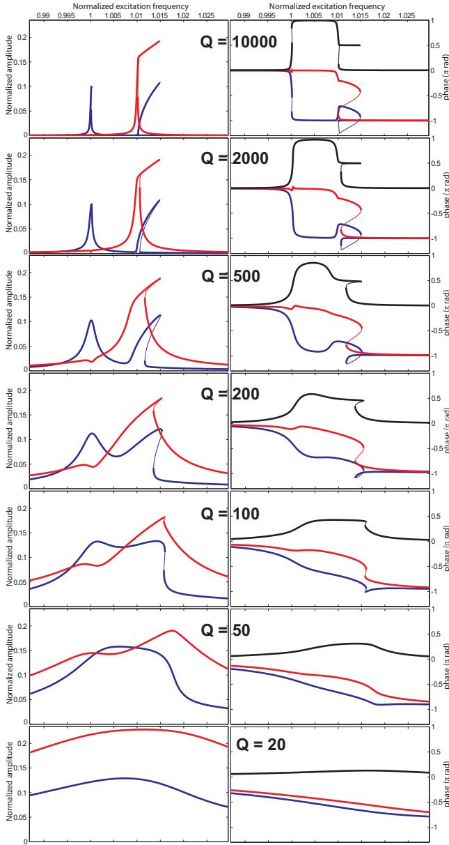
FIG. 7. Evolution of the elliptical transition as the quality factor decreases. The frequency difference is set to 1% and the excitation is increased to have Q \cdot F = \text{constant} .
