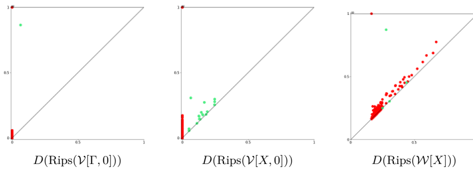
■ Figure 5 Persistence diagrams of some simplicial filtrations. Points in red (resp. green) represent the persistent homology in dimension 0 (resp. 1).
