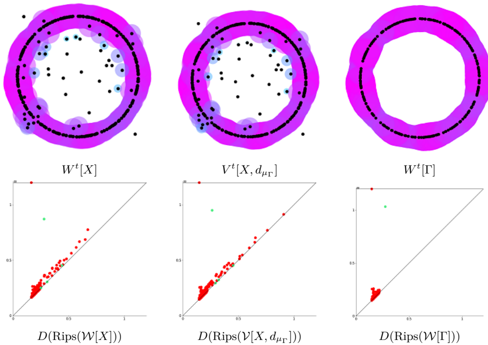
■ Figure 6 Filtrations for t = 0.4 , and their corresponding persistence diagrams.
