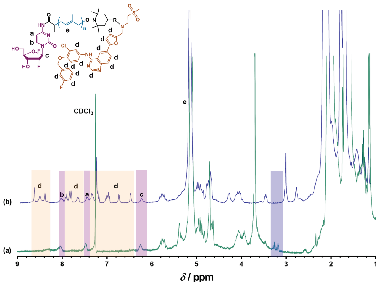
Figure 5. Representative ^1\text{H} NMR spectrum in \text{CDCl}_3 in the 1–9 ppm region of (a) Gem-PI-SG1 ( G2 ) and (b) Gem-PI-Lap ( G2L ), with \text{R} = \text{succinate} . After nitroxide exchange with TEMPO-Lap, the proton signals from Lap (brown areas) appeared, those from Gem are retained (purple areas) and those from SG1 (blue area) disappeared.
