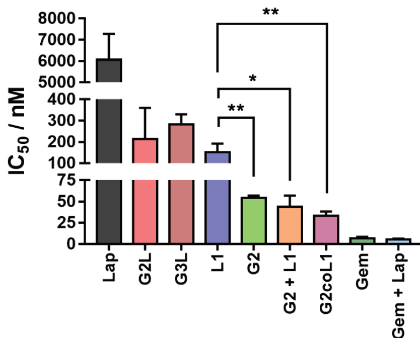
Figure 9. IC 50 values \pm SD of Gem-PI-Lap ( G2L-G3L ), Gem-PI ( G2 ), PI-Lap ( L1 ), Gem-PIcoPI-Lap ( G2coL1 ), Gem-PI + PI-Lap ( G2+L1 ) nanoparticles, free Gem, free Lap and free Gem + Lap (1:1, mol:mol) determined by MTT test on MCF-7 cells after 72 h of incubation. (** p < 0.01 G2coL1 vs G2 or L1 , * p < 0.05 G2+L1 vs L1 ).
