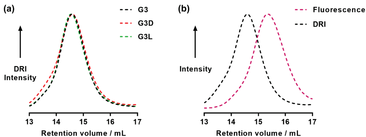
Figure 3. Size exclusion chromatograms ( \text{CHCl}_3 eluent, 1 \text{ mL}\cdot\text{min}^{-1} ) of (a) Gem-PI-SG1 ( G3 , black dashed line), Gem-PI-Dox ( G3D , red dashed line) and Gem-PI-Lap ( G3L , green dashed line) and (b) Gem-PI-Dox ( G3D ) fluorescence (purple dashed line) and DRI (black dashed line) after nitroxide exchange (the gap in retention volume between DRI and fluorescence traces comes from the tubing between the two detectors).
