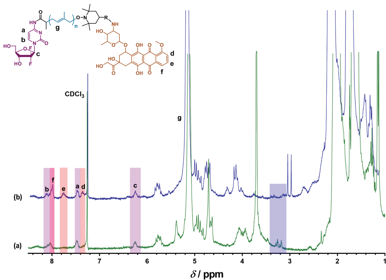
Figure 4. Representative 1 H NMR spectrum in CDCl 3 in the 1–8.5 ppm region of (a) Gem-PI-SG1 (G2) and (b) Gem-PI-Dox (G2D), with R = succinate. After nitroxide exchange with TEMPO-Dox, the proton signals from Dox (red areas) appeared, those from Gem are retained (purple areas) and those from SG1 (blue area) disappeared.
