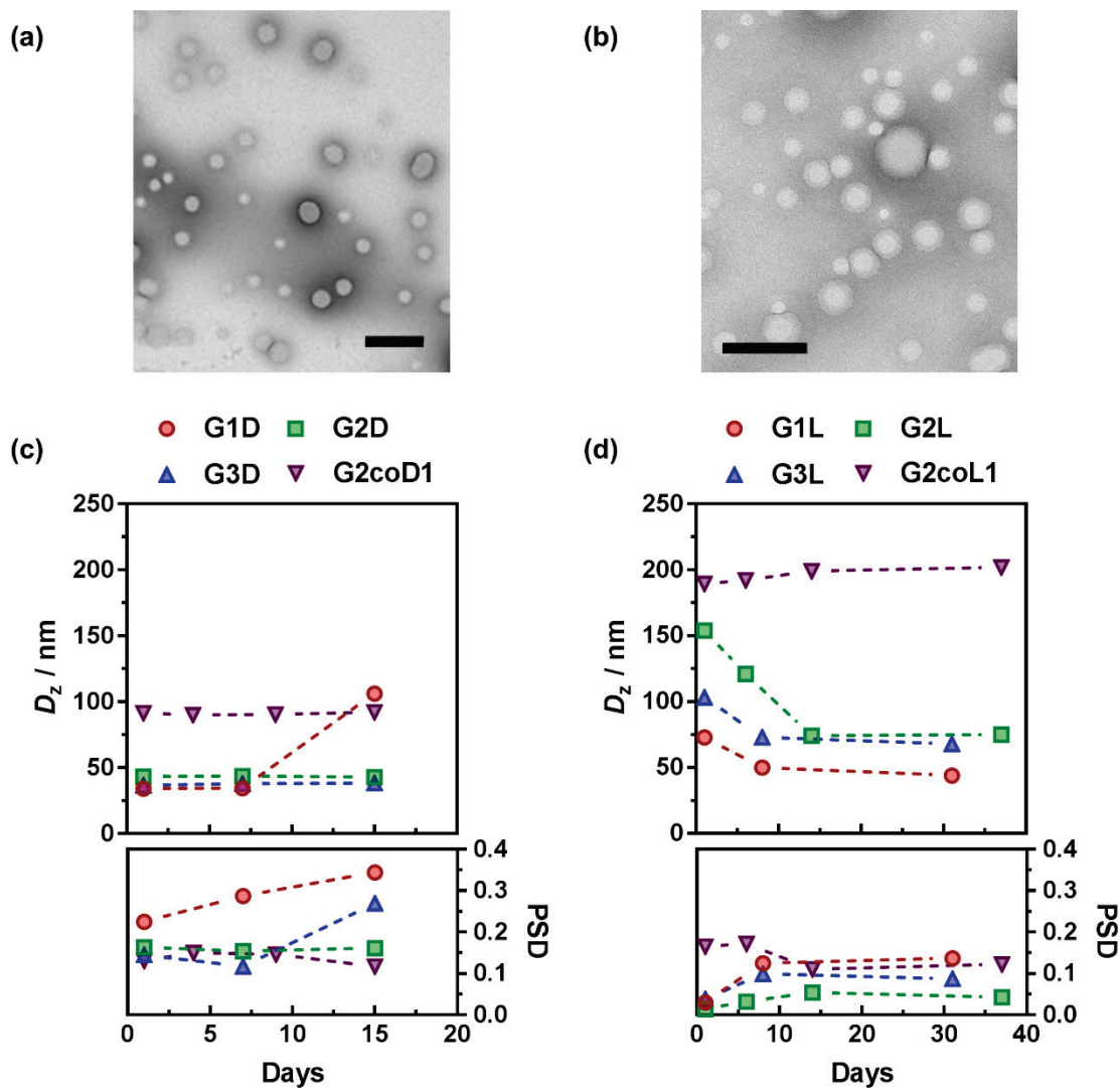
Figure 6. Representative TEM images of (a) Gem-PI-Dox nanoparticles G3D (scale bar = 1 \mu\text{m} ) and (b) Gem-PI-Lap nanoparticles G2L (scale bar = 0.5 \mu\text{m} ). Evolution of the average diameters ( D_z ) and the particle size distributions (PSD) measured by DLS in water of (c) Gem-PI-Dox nanoparticles ( G1D , G2D , G3D and G2coD1 ) and (d) Gem-PI-Lap nanoparticles ( G1L , G2L , G3L and G2coL1 ).
