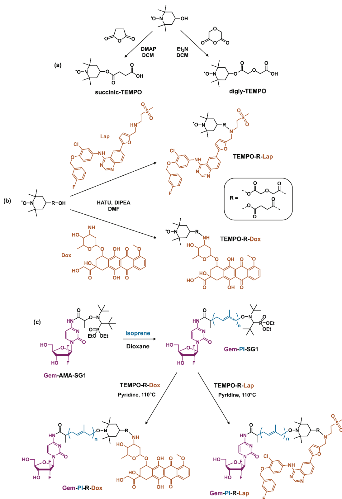
Scheme 1. (a) Synthesis of succinic-TEMPO and digly-TEMPO. (b) Synthesis of TEMPO-R-Dox and TEMPO-R-Lap. (c) Synthesis of heterobifunctional Gem-PI-R-Dox and Gem-PI-R-Lap polymer prodrugs by “ drug-initiated ” nitroxide-mediated polymerization (NMP) of isoprene from Gem-AMA-SG1 followed by nitroxide exchange from TEMPO-R-Dox and TEMPO-R-Lap. PI = polyisoprene, Gem = gemcitabine, Dox = doxorubicin and Lap = lapatinib.
