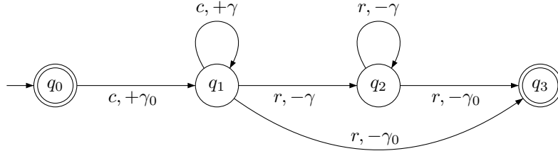
Figure 4: VPA A_3 on \Sigma_c = \{c\} and \Sigma_r = \{r\} .
