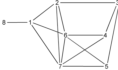
Figure 2: The graph G(\mathcal{T}) for \mathcal{T} in Figure 1.
