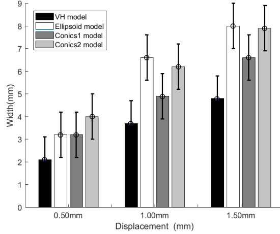
Fig. 7. Width of the contact area for plane contact compression at 20^\circ from simulations with the VH , Ellipsoid , Conics1 and Conics2 models
