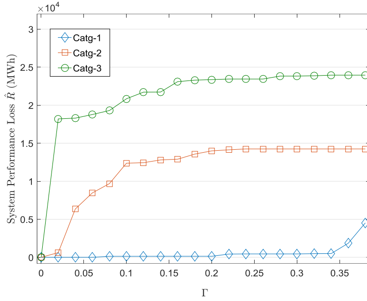
Fig. 5. Optimized worst case load shedding (system performance loss \hat{R} ) under different failure uncertainty \Gamma at \Upsilon = 0.1 .
