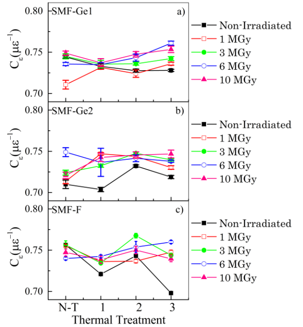
Fig. 4 Strain coefficients in non-thermally treated and treated SMF-Ge1 (a), SMF-Ge2 (b) and SMF-F (c). We report C_ε of non-irradiated (black points), 1 MGy (red points), 3 MGy (green points), 6 MGy (blue points) and 10 MGy (pink points) irradiated samples.
