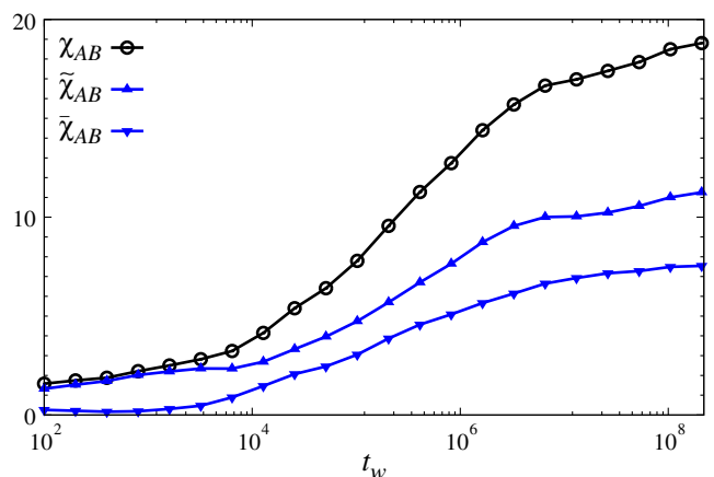
FIG. 5. Time evolution of the susceptibilities at Z = 1000 . The total susceptibility \chi_{AB} is decomposed into sample-to-sample fluctuations \bar{\chi}_{AB}(t_w) and clone-to-clone fluctuations within each individual sample \tilde{\chi}_{AB}(t_w) . Both contributions are comparable in amplitude and time evolution.
