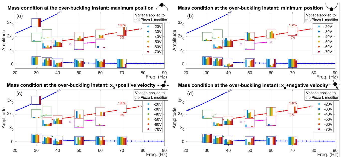
Figure 10: Experimental results of orbit jump trials by modification of the length L showing the steady-state behaviors stabilized after the trials. Each colored stick inside the boxes corresponds to the number of trials leading to the behavior given by the position of the box. The bottom and the top of the boxes respectively correspond to 0 and 30 trials ( i.e. , 0% and 100% of the trials).
