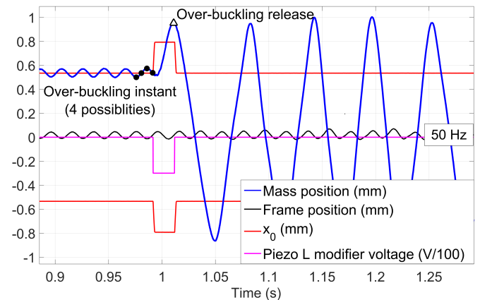
Figure 9: Experimental time signal example of an orbit jump trial by modifying the length L (i.e., the buckling level).
