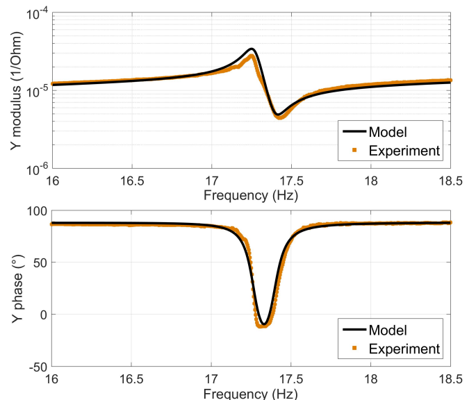
Figure 7: Magnitude and phase of the prototype admittance and its fitted model for the identification of parameters (\omega_0, Q, C_0, \alpha) .
