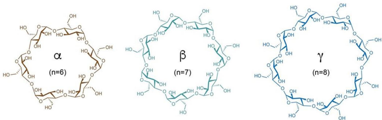
Figure 3: The chemical structure of the most common native cyclodextrins.
