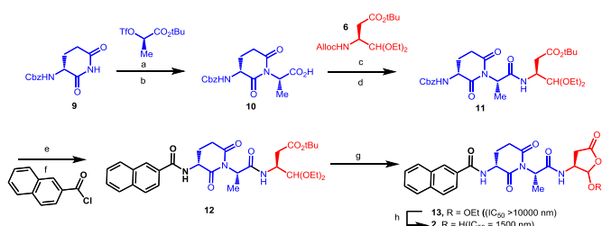
Scheme 2. A representative route designed for P4 exploration and used to deliver eg., 2 . Reagents and conditions: (a) K 2 CO 3 , MeCN, r.t., 53%; (b) TFA, 0 °C-r.t., quant.; (c) Pd(PPh 3 ) 4 , DMBA, DCM, r.t., 15 min; (d) 10 pre-activated EDCl, HOBT, DCM, DMF, 0 °C, 15 min, amine from step (c) added, r.t., 16 h, 62%; (e) H 2 , Pd(OH) 2 -C, EtOAc, r.t., 78%; (f) TEA, DCM or 43%; (g) TFA, DCM, r.t., 75%; (h) 2N HCl (aq), MeCN, 0 °C-r.t., 52%.
