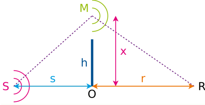
Figure 13: Simple case of diffraction method.
