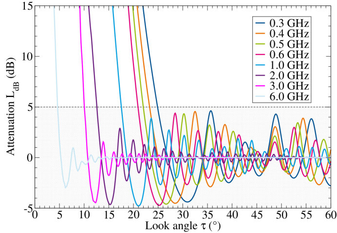
Figure 9: Attenuation in dB obtained by the FEM method for different frequency values.
