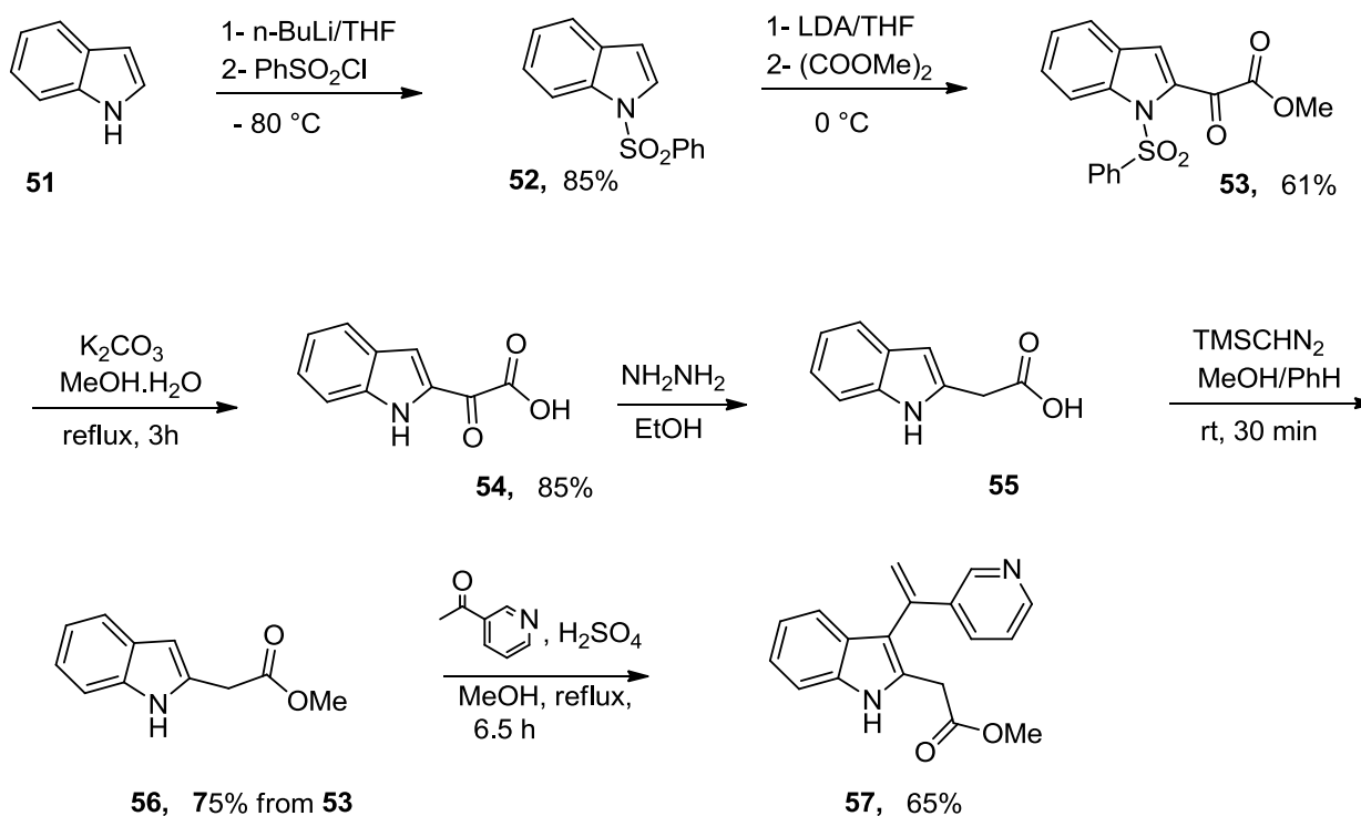
Scheme 12. Synthesis of 57 .
