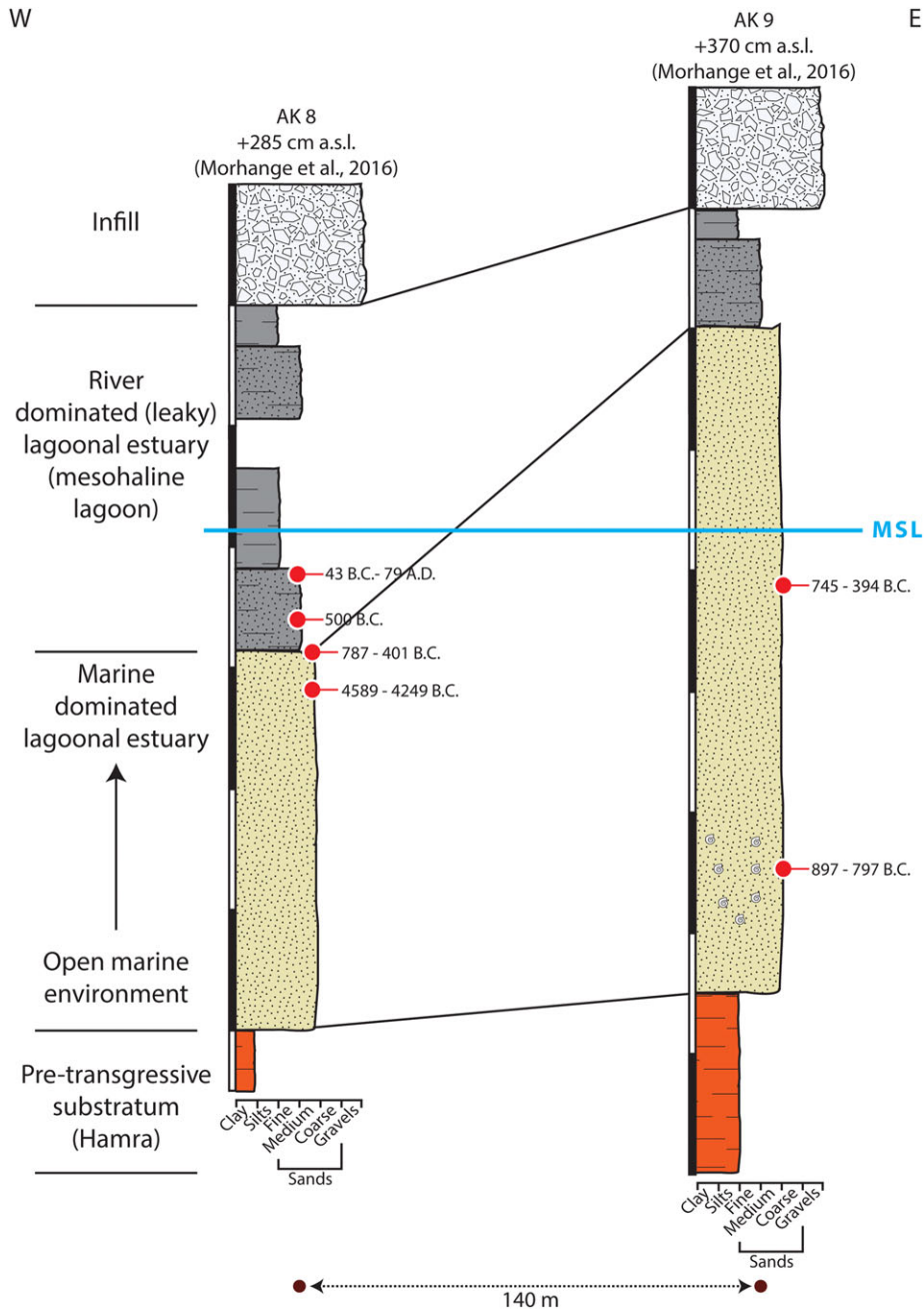
FIGURE 8 East–West transect in the southern part of Tel Akko (cores AK 8 and AK 9 after Morhange et al., 2016) Notes. The location of the cores is given in Figure 3. [Color figure can be viewed at wileyonlinelibrary.com ]
