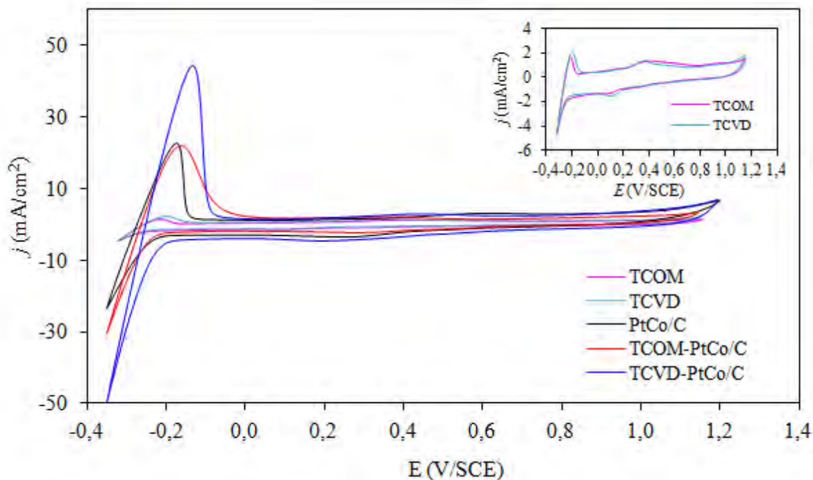
Figure 5. Representative cyclic voltammetry of PEM fuel cells with pure \text{TiO}_2 and fresh \text{TiO}_2\text{-PtCo/C} catalysts in \text{N}_2 -saturated 0.5 \text{ M H}_2\text{SO}_4 at scan rate of 20 \text{ mV/s} .
