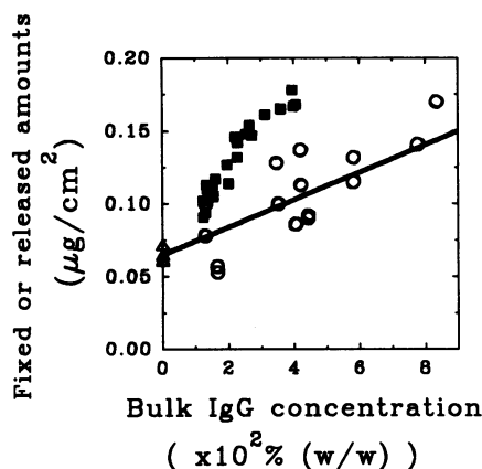
FIG. 5. \circ , Released amounts of labeled IgG* ( \Delta\Gamma_{r+} ) from latex particles (saturated with IgG*) versus c_{IgG} at a constant reaction time of 4 hr. \Delta , Pure desorption experiments ( c_{IgG} \approx 0 ). Solid line was calculated from the kinetic law deduced from Fig. 4 with k_e f(\Gamma_{IgG, Tot}) = (2.3 \pm 0.4) \times 10^{-5} \text{cm} \cdot \text{hr}^{-1} and a y intercept of 0.06 \mu\text{g} \cdot \text{cm}^{-2} . \blacksquare , Fixed amounts of labeled IgG* ( \Delta_{IgG^*} ) versus c_{IgG^*} at the same reaction time. Data include the values from the 10 kinetics measurement (set I) and from 11 additional measurements (see text).
