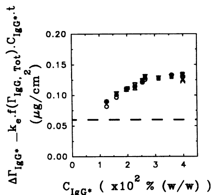
FIG. 6. Calculated values of \Delta\Gamma_{IgG^*} - k_e f(\Gamma_{IgG, Tot}) \cdot c_{IgG^*} \cdot t , for the different reaction times with the experimental data from set I, versus c_{IgG^*} . Symbols \circ , \square , \Delta , \bullet , and \nabla correspond to the reaction at 2, 3, 4, 4.5, and 5 hr, respectively. Dashed line shows the amount of labeled molecules that replaced the desorbed ones ( 0.06 \mu\text{g} \cdot \text{cm}^{-2} ; see Fig. 5). X, Additional experiments performed according to set I with only labeled molecules (see text).
