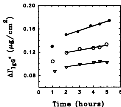
FIG. 3. Examples of kinetic experiments according to set I. \Delta\Gamma_{\text{IgG}^*} , surface concentration of labeled IgG* for various bulk concentrations c_{\text{IgG}^*} : \nabla , (1.22 \pm 0.05) \times 10^{-2}\% ; \circ , (1.97 \pm 0.05) \times 10^{-2}\% ; \bullet , (3.60 \pm 0.10) \times 10^{-2}\% . Straight lines correspond to least-squares fits in the interval 2–5 hr.
