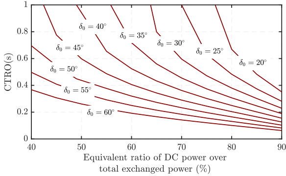
Fig. 7: CRTO as function of the initial angle \delta_0 and the ratio of HVDC transmitted power over the total exchanged power between regions. Complete loss of the HVDC power and H = 6s
