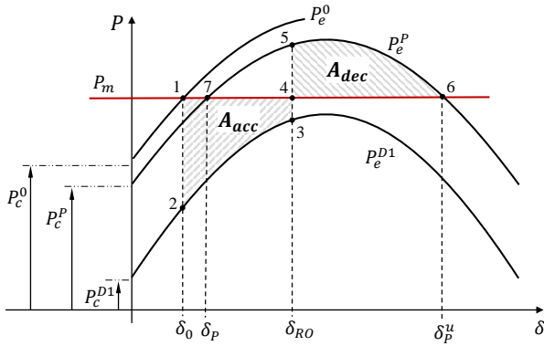
Fig. 3: AC/DC Equal area criterion in case of DC fault
