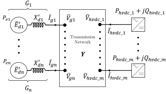
Fig. 1: Multi-machine/multi-converter power system
