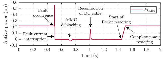
Fig. 4: AC side power injections of the faulted pole of station 1 during a DC fault using the Converter-Breaker strategy
