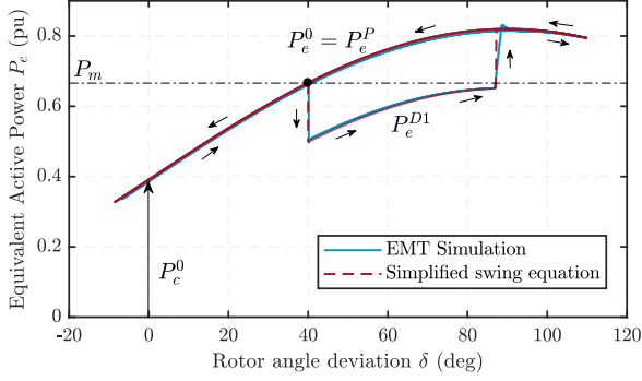
Fig. 5: Validation of AC/DC Equal area criterion
