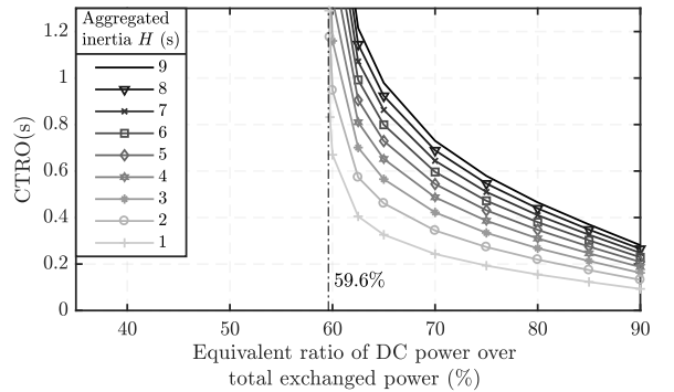
(b) 50% of the HVDC power is lost (Bipolar configuration)
