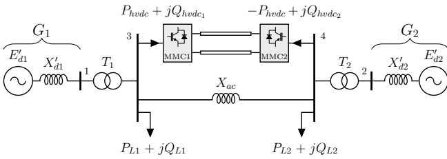
Fig. 2: 2-Area 2-Machine AC/DC power system
