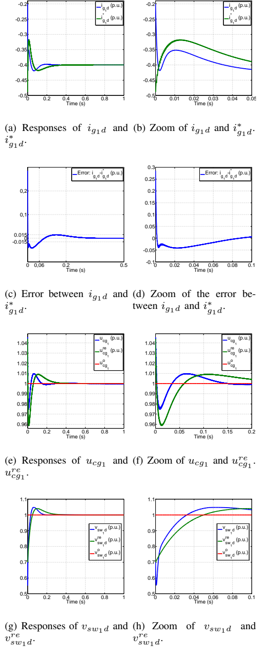
Fig. 4. Simulation results with the control gains in Set 1.
