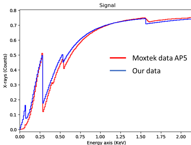
717 718 Fig. Comparison of the modelled detector efficiency curve using Love and Scott model and the AP5 curve 719 proposed by moxtek ©.
