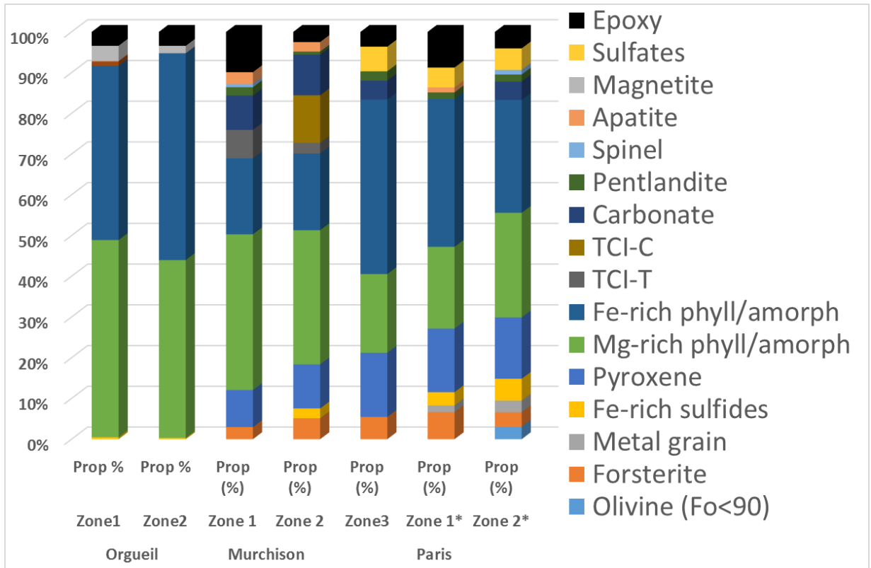
566 567 Fig 9: Modal mineralogy of the different matrices as determined by phase mapping and MLLS fitting. For phases 568 other than phyllosilicates, relative errors range from 0.5 to 3%. This error is larger for phyllosilicates (8-12 %). Zones 569 with a symbol "*" indicate areas from which large chondrule fragments were ignored (see supplementary materials 6). 570
