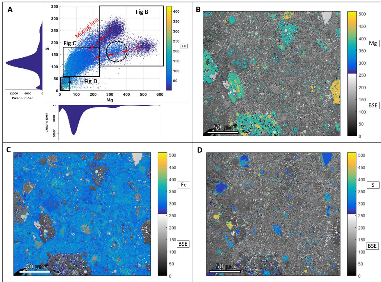
375 Fig 3: A: X-ray intensities of Mg and Si peaks, combined with Fe intensity (colorbar). Each point corresponds to one pixel (Paris Zone 2). Pixels of identical composition form clusters. B: forsterite and enstatite map based on the selection of the corresponding cluster. C: This cluster corresponds to a fine-grained mixture of amorphous silicates, phyllosilicates with sulfides and anhydrous silicate inclusions. D: Map of the remaining pixels after thresholding for Mg and Si. This selection contains Mg and Si-free phases, such as metal grains, sulfides, etc. Unselected pixels are displayed as a secondary electron image or back-scattered electron image.
