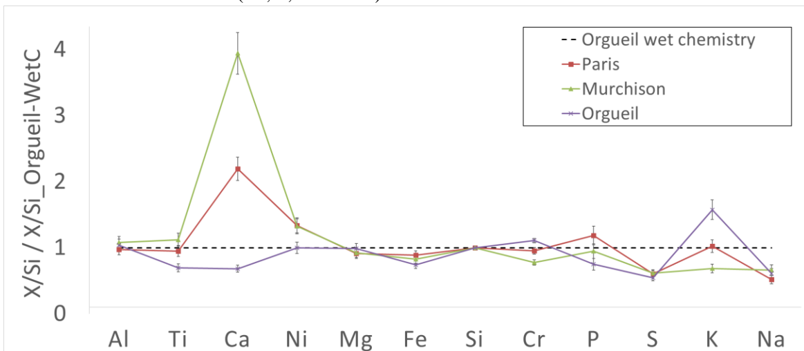
574 575 Fig 10: Bulk compositions of matrices (atomic ratios) calculated by ACADEMY (average of all analyzed regions) 576 normalized to silicon and to the composition of Orgueil determined by wet chemistry (Lodders & Palme, 2009). (See 577 supplementary materials 7)
