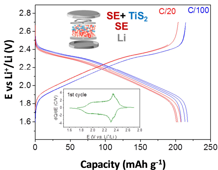
Figure 5. Electrochemical galvanostatic discharge/charge cycling with \text{TiS}_2 electrode with \text{Li}(\text{BH}_4)_{0.75}\text{I}_{0.25}+(\text{Li}_2\text{S})_{0.75}+(\text{P}_2\text{S}_5)_{0.25} solid electrolyte at 50^\circ\text{C} (Inset: dQ/dE curve for the first cycle) [27].
