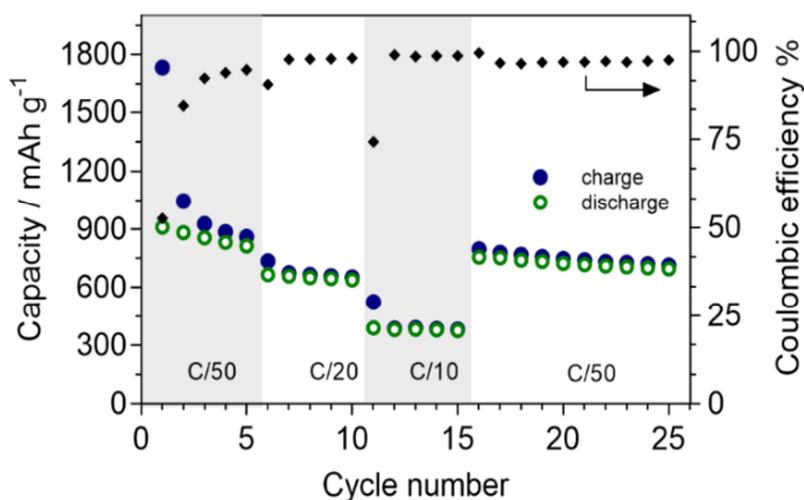
Figure 8. Charge/discharge profiles at different C rates (C/50, C/20 and C/10 then C/50 again, five cycles each) of the complete solid-state battery \text{Li}_2\text{S}+\text{LiBH}_4+\text{KB}|\text{LiBH}_4|\text{MH}+\text{LiBH}_4+\text{C65} at 120 °C [35].
