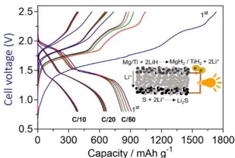
Figure 7. Charge/discharge profiles at different C rates (C/50, C/20 and C/10, five cycles each) of the complete ASS battery \text{Li}_2\text{S}+\text{LiBH}_4+\text{KB}|\text{LiBH}_4|\text{MH}+\text{LiBH}_4+\text{C65} at 120^\circ\text{C} and schematic representation of the discharge redox reaction [33].
