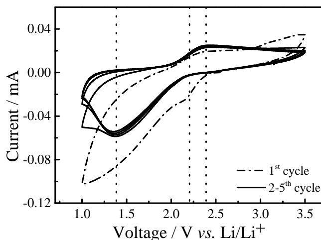
Figure 3. Cyclic voltammogram (at 55 °C and scan rate of 0.1 mV s -1 ) of a solid-state Li|LiBH 4 @SiO 2 |S+C battery based on a LiBH 4 -SiO 2 nanocomposite electrolyte [17].
