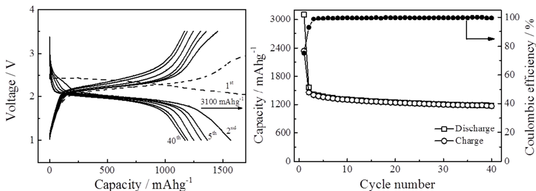
Figure 4. Cycling performance and discharge /charge capacity and Coulombic efficiency of a solid-state Li-S battery based on LiBH 4 -SiO 2 nanocomposite as electrolyte, measured at 55 °C, current density of 6.2 μA cm -2 , corresponding to C-rates of 0.03 C, and with cut-off voltages of 1 and 3.5 V [17].
