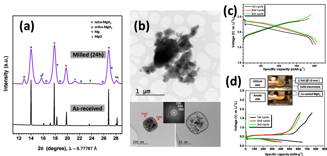
Figure 1. PXD patterns (a) and bright field TEM micrographs (b) of the 24h-milled \text{MgH}_2 under \text{H}_2 atm. (Inset: Fourier transform of the bright field TEM image); RT discharge-charge (3 first cycles, 30 °C, 0.01 \text{ mA cm}^{-2} )
