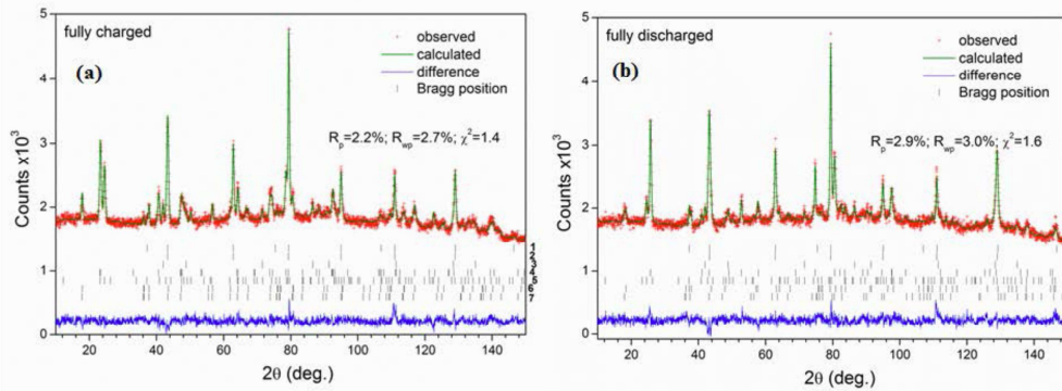
Figure 9. Neutron diffraction patterns for the fully charged (a) and discharged (b) battery along with the results of the Rietveld refinements. Phase constituents, from bottom to top: (a) \text{Li}_{0.2}(\text{Ni,Mn,Co})\text{O}_2 , \text{Li}_{0.4}\text{CoO}_2 , \text{LiC}_{12} , \text{LiC}_6 , Cu, Fe, Al; (b) \text{Li}(\text{Ni,Mn,Co})\text{O}_2 , \text{LiCoO}_2 , \text{LiC}_{12} , C, Cu, Fe, Al.
