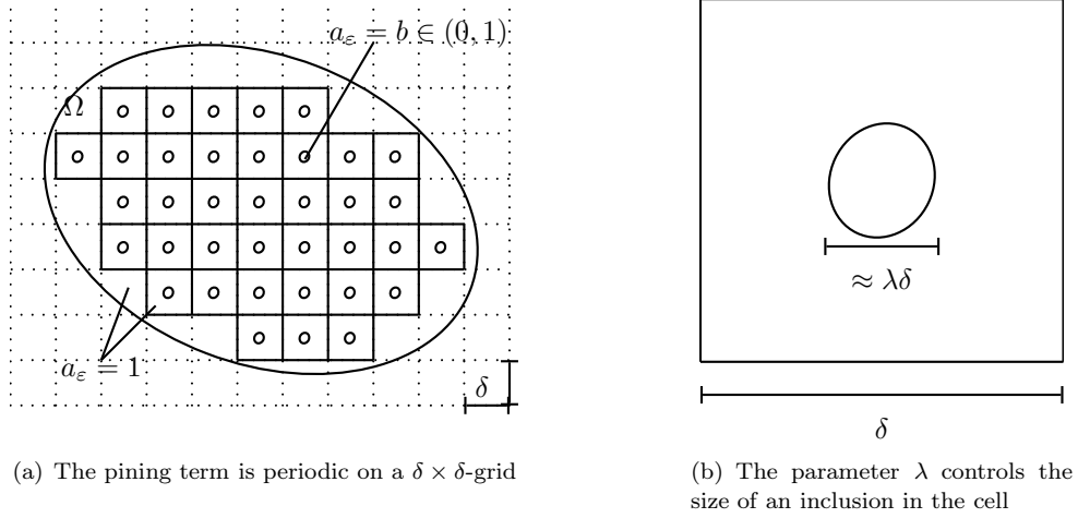
FIGURE 1. The periodic pinning term
