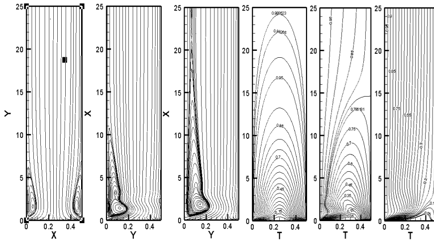
Figure 5: Stream lines and isothermal lines for different temperature cases T_2=1,0.8,0.1 .
