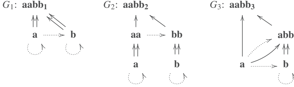
Figure 4. Three different structural universals specializing being aabb .
