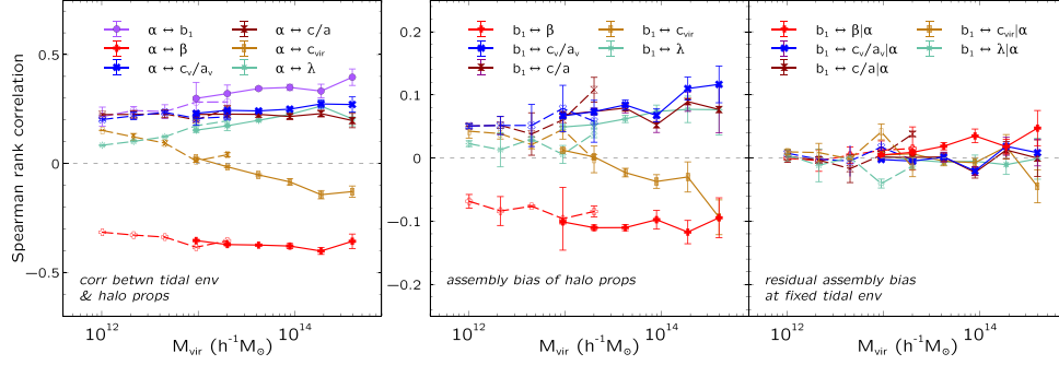
Figure 2. Correlations between internal halo properties, tidal environment, and large-scale bias. (Left-hand panel): Spearman rank correlation coefficients, for haloes in bins of mass M_{\text{vir}} , between tidal anisotropy \alpha and other halo properties, including \gamma_{\alpha b_1} with large-scale bias b_1 and \gamma_{\alpha c} with internal properties c \in \{\beta, c_v/a_v, cla, c_{\text{vir}}, \lambda\} (see caption of Fig. 1). In the legend, each coefficient \gamma_{ab} is represented by the symbol a \leftrightarrow b . (Middle panel): Assembly bias trends seen using Spearman rank correlation coefficients \gamma_{b_1 c} between halo bias and each internal property c (cf. Fig. 1). (Right-hand panel): Conditional correlation coefficients \gamma_{b_1 c|\alpha} (equation 12) for each internal property c . Note that the vertical axis in the middle and right-hand panels is zoomed in by a factor approximately three as compared to the left-hand panel. The formatting of symbols (filled versus empty) and lines (solid versus dashed) is identical to that in Fig. 1. The right-hand panel shows the main result of this work: each conditional coefficient \gamma_{b_1 c|\alpha} is substantially smaller in magnitude than the corresponding unconditional coefficient \gamma_{b_1 c} in the middle panel. Thus, conditioning on tidal anisotropy \alpha largely accounts for the assembly bias trend of all internal halo properties. See the text for a discussion.
