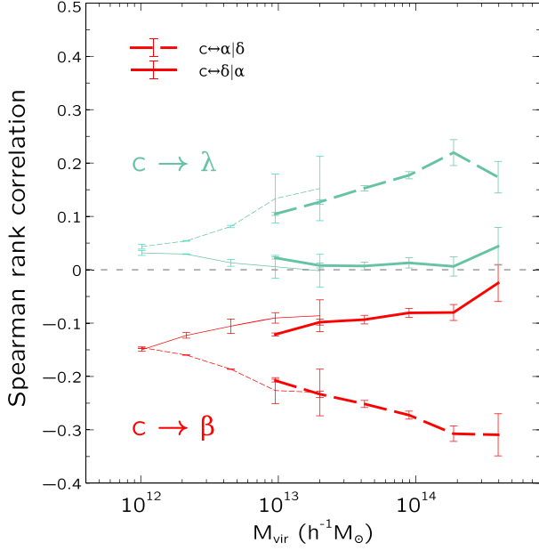
Figure A4. Correlation between tidal environment at 4R_{200b} scales (as measured by \alpha and \delta ) and internal halo properties c \in \{\beta, \lambda\} . The curves show the conditional coefficients \gamma_{c\delta|\alpha} (solid) and \gamma_{c\alpha|\delta} (dashed). We see that |\gamma_{c\delta|\alpha}| < |\gamma_{c\alpha|\delta}| at essentially all masses in both cases, indicating that \alpha accounts for a substantial fraction of the correlation of \delta with both of these internal properties. We find qualitatively similar results for the other internal properties \{c_v/a_v, c/a, c_{vir}\} (not shown).
