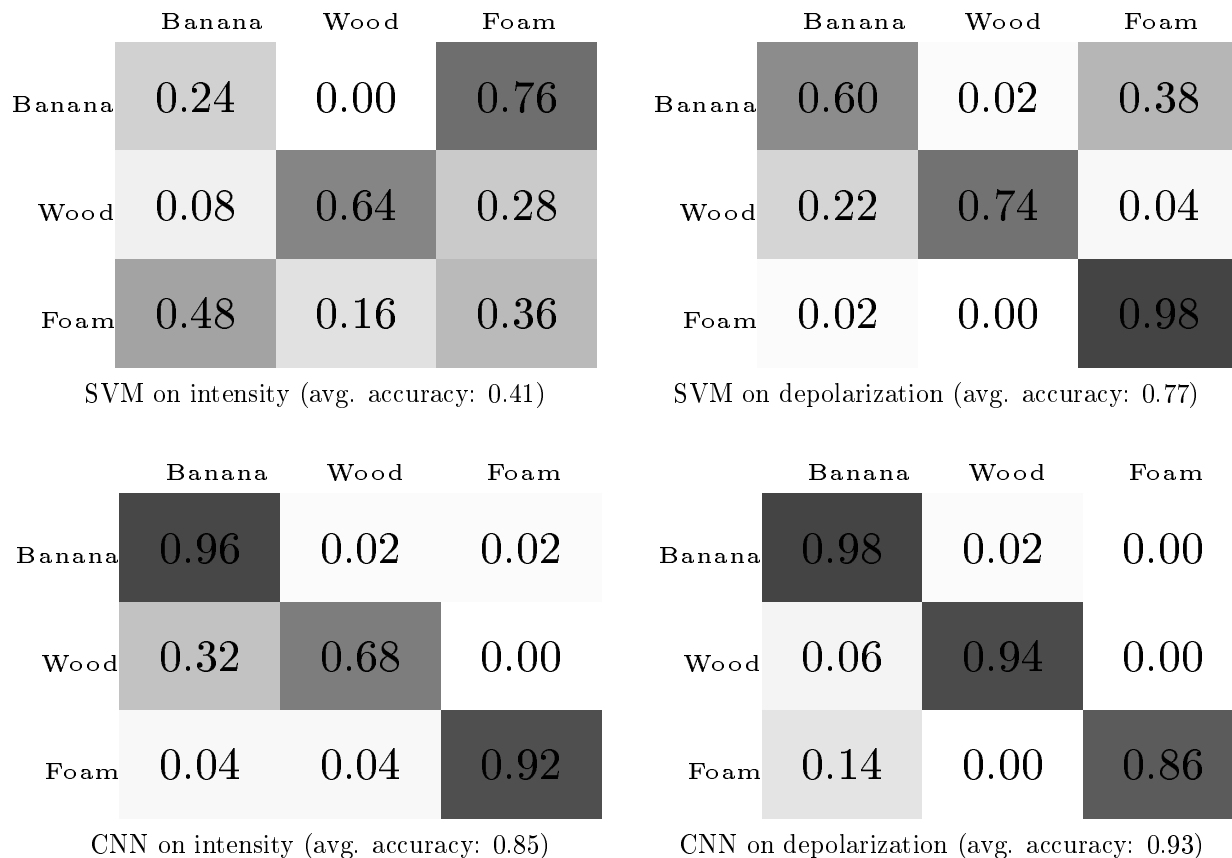
Figure 5. Confusion matrices obtained for the classification of real-world banana, wood and foam samples, using Matlab’s builtin support vector machine (SVM) classifier 15 with default parameters (top) or a state-of-the-art convolutional neural network (CNN) 13 whose parameters are initialized by pretraining on the ImageNet database 16 (bottom), on intensity (left) and depolarization (right) images. In each table, the columns show the predicted labels, the rows show the true labels and the numbers indicate the percentage of classifications. Considering depolarization instead of intensity improves the results in both cases: standard image classification tools can thus readily be applied to active polarimetric imaging systems and classification seems to benefit from the use of polarimetry-aware data.
