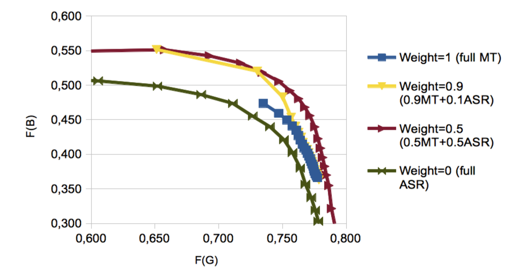
FIGURE: WCE performance (F(B) vs F(G)) of different WCE methods - for SLT - for different decision thresholds varying from 0.5 to 0.9).
