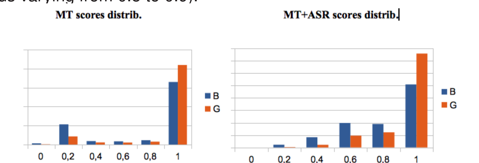
FIGURE: Evolution of the WCE scores distribution from MT features to MT+ASR features
