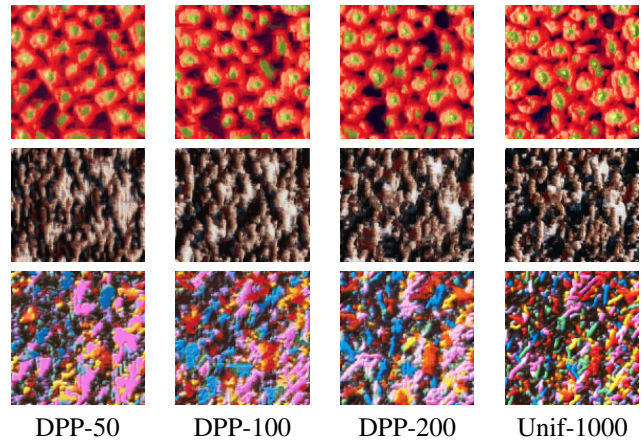
FIGURE 2 – Setting the Expected Cardinal of the DPP. In this figure we display the impact on the visual results of the expected cardinal of the DPP. See the text for comments.
