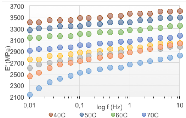
Fig.3a:Storage modulus vs frequency
