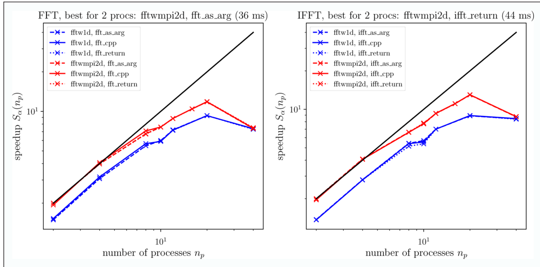
Figure 8: Speedup computed from the median of the elapsed times for 2D fft ( 2160 \times 2160 ) at LEGI on cluster8.
