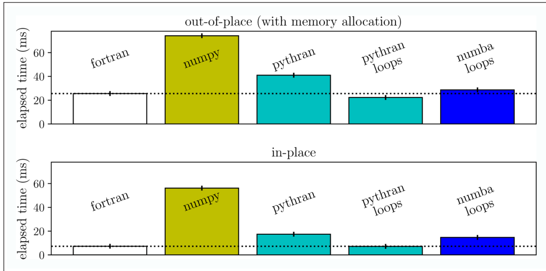
Figure 9: Elapsed time (smaller is better) for the projection function for different implementations and tools. The shape of the arrays is (128, 128, 65) . The dotted lines indicate the times for Fortran for better comparison.
