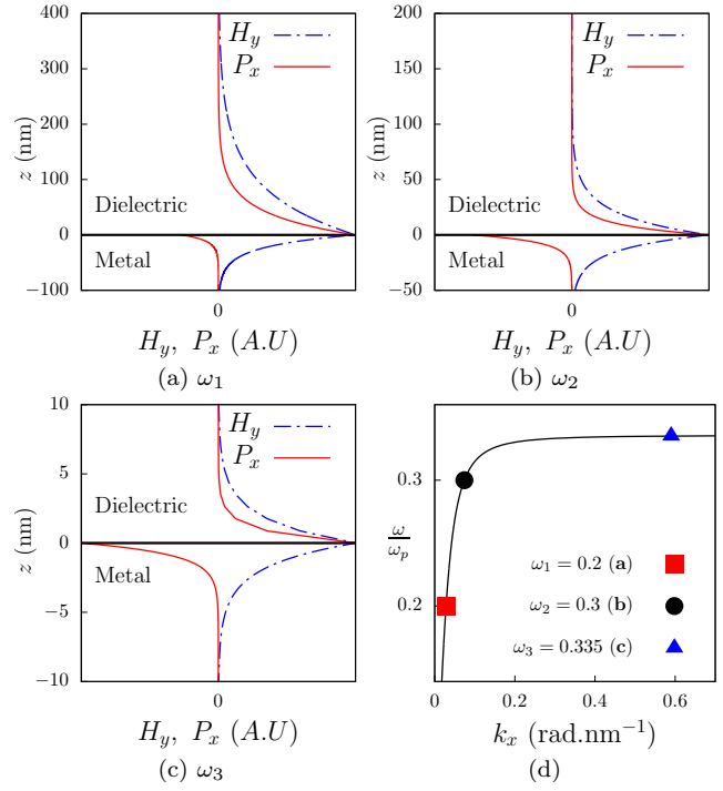
Fig. 1. (a), (b), (c) Magnetic field and Poynting vector profiles in the case of the surface plasmon for different values of \frac{\omega}{\omega_p} . (d) Dispersion curves for the surface plasmon, showing the frequencies \omega_1 , \omega_2 and \omega_3 .
