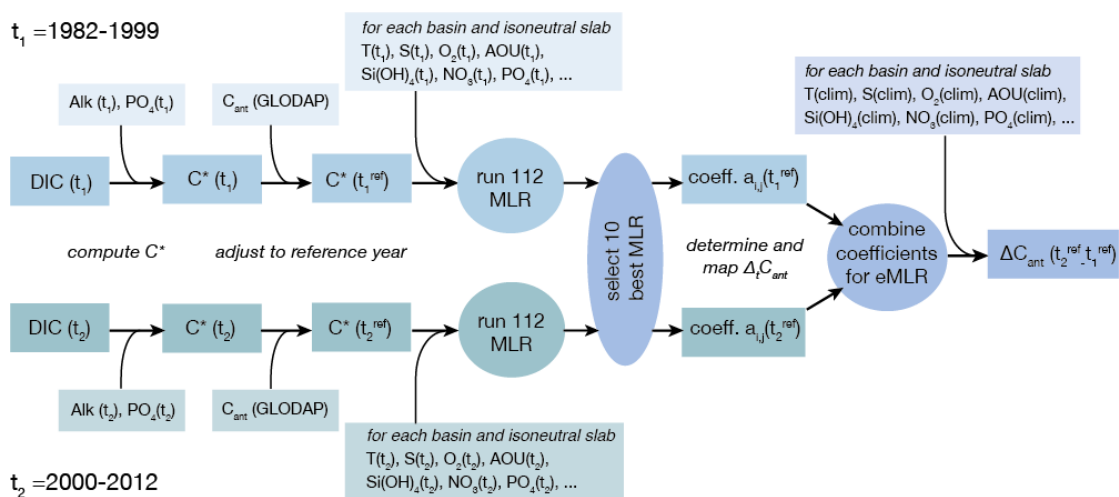
Figure S3: Procedure to estimate the change in anthropogenic CO 2 between the JGOFS/WOCE and the GOSHIP eras in the water column below 150 m. Adapted from ref(9).
