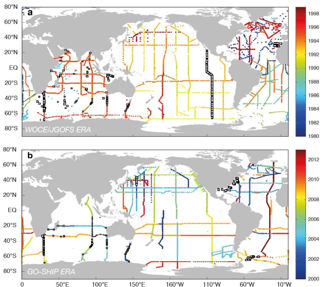
Figure S1: Maps of the sampling locations of the data used for the two eras: (a) for the WOCE/JGOFS era (1982 to 1999) and (b) as (a), but for the Repeat Hydrography/GO-SHIP era (from 2000 to 2013). The colors of the filled dots indicate the year of sampling. Open squares indicate stations/cruises that are in GLODAPv2, but not used for our analyses (see text for details). The size of the squares indicates the number of samples affected: Small: 0-9 samples, Medium: 10-19 samples, Large >19 samples. Stations that were sampled more than once during the Repeat Hydrography/GO-SHIP era are shown with two colors and with the second occupation plotted on top.
