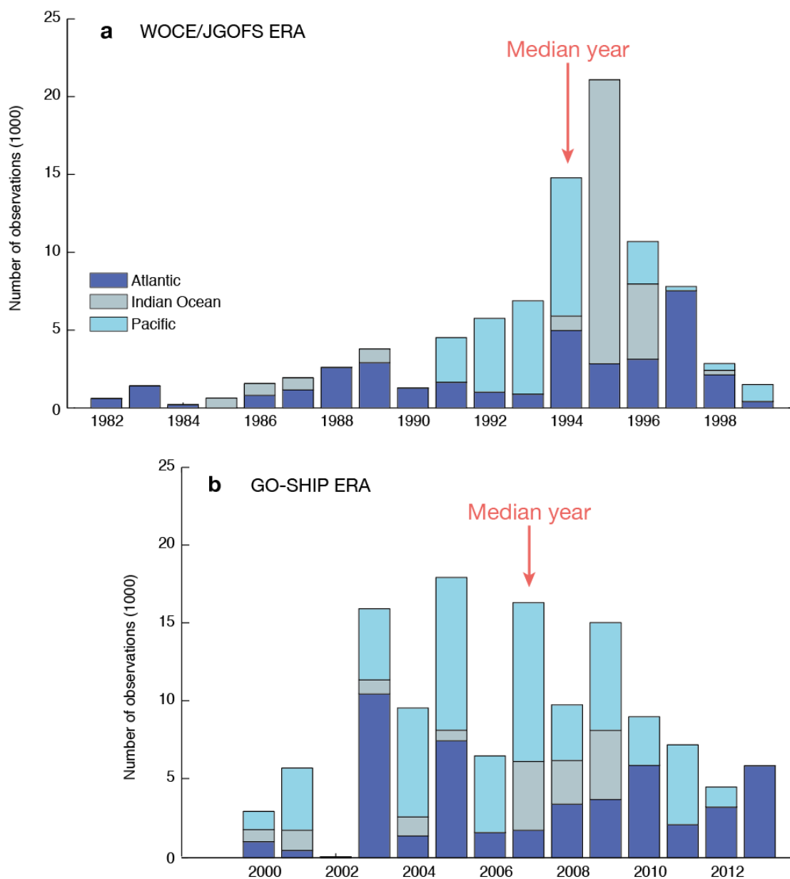
Figure S2: Distribution of the data through time. Shown are the number of discrete samples of C* for each year and basin that were used to construct the two multiple linear regression models.
