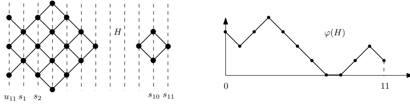
FIGURE 7. The heap of a FC involution in \tilde{\mathcal{C}}_{11} and its associated walk.
