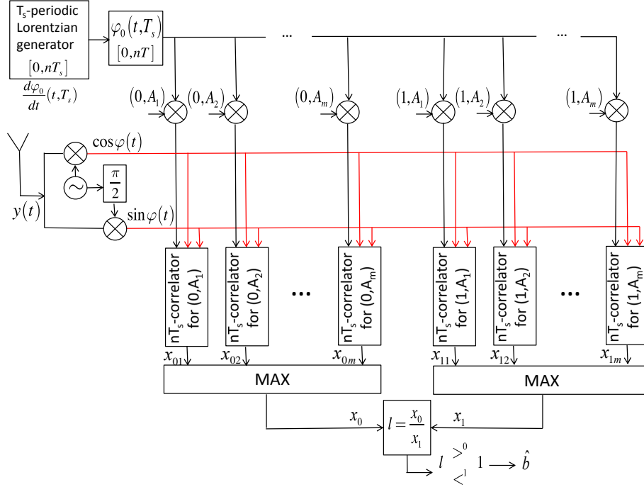
Figure 4: Block diagram of the AMF-based detector.
