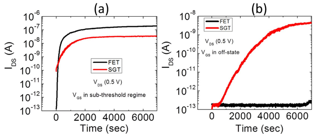
Figure 8. The drain current through the SGT and FET devices during the continuous stress applied for more than 100 min: (a) in s-s regime, and (b) off-state of transistor.
