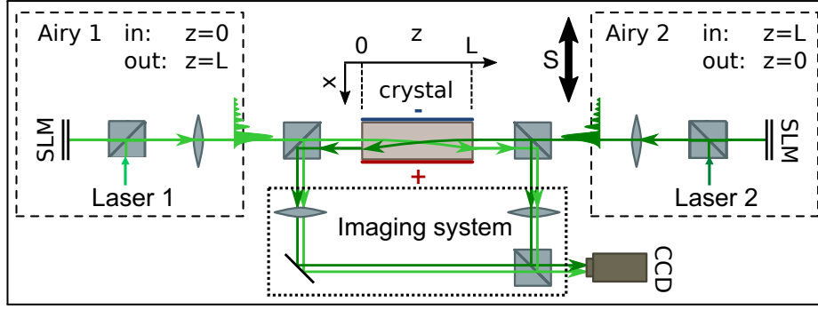
Figure 1. (Color online) Study of two incoherent CP Airy beams in a biased focusing photorefractive (PR) crystal: experimental setup.
