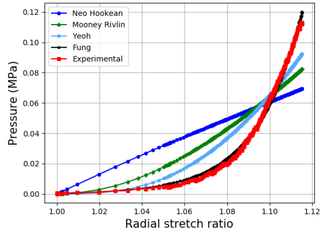
Figure 2: Example of inverse identification with 4 constitutive models
