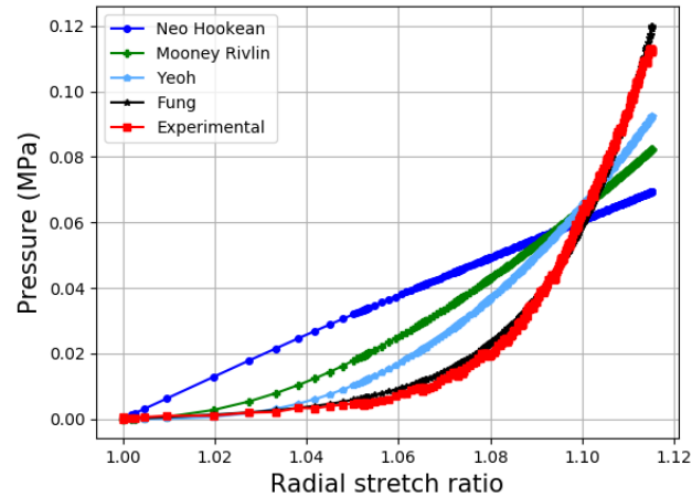
Figure 2: Example of inverse identification with 4 constitutive models
