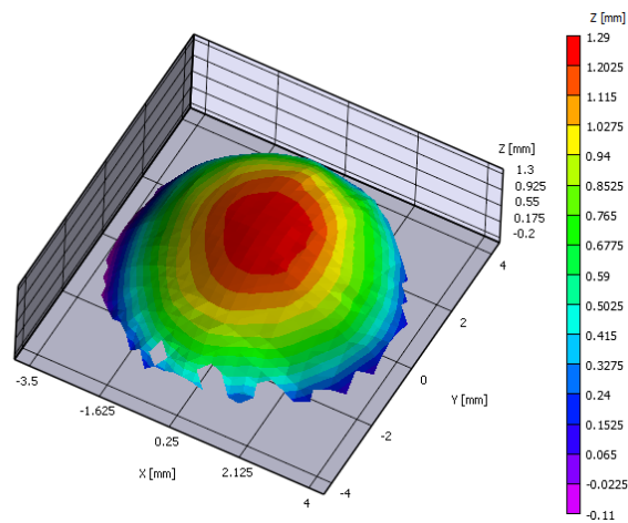
Figure 1 : 3D surface of a diaphragm sample VIC 3D ©.
