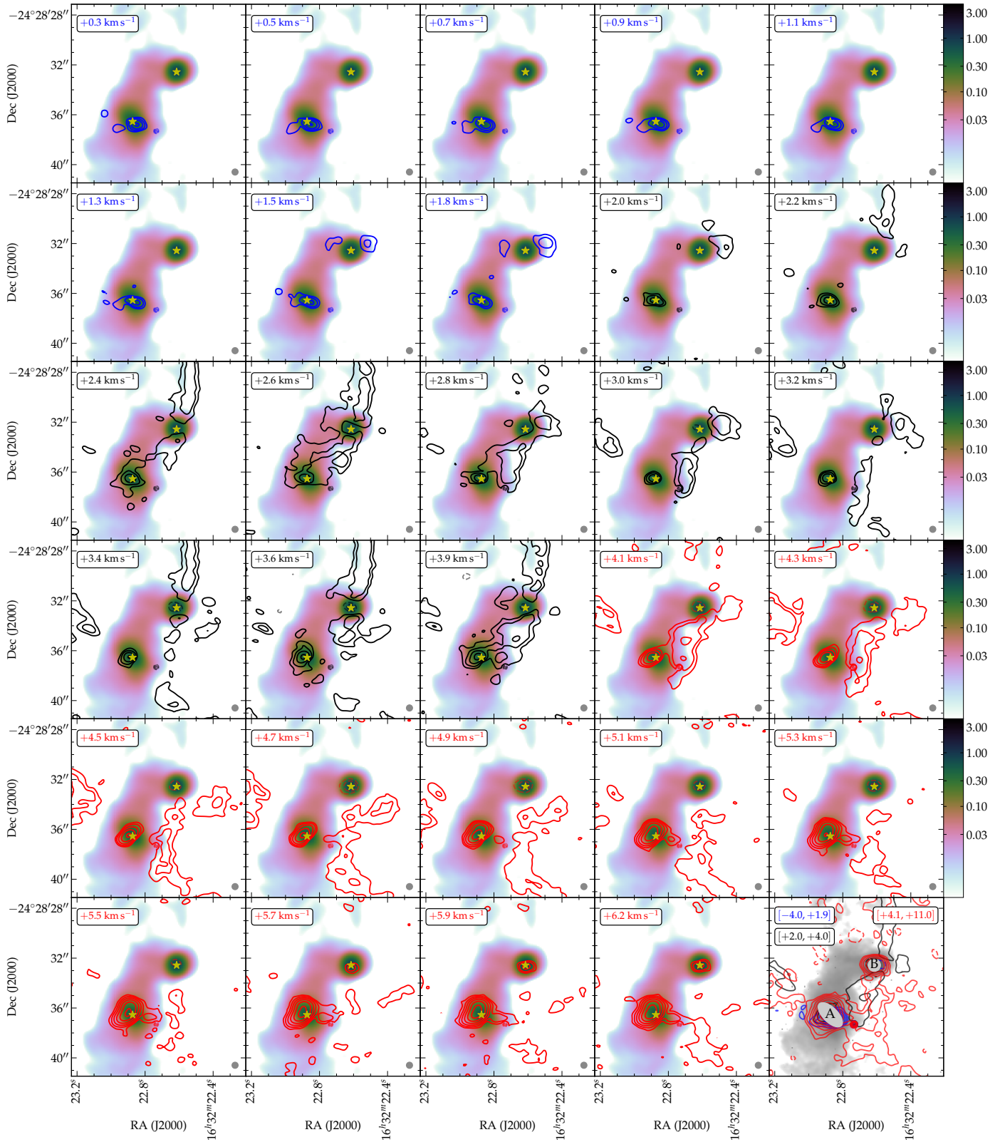
Fig. B.8. C_2H channel maps. As Fig. B.1. First positive (negative) contour level in individual channel maps: 0.03 ( -0.06 ) \text{Jy beam}^{-1} ; first contour levels in the bottom right integrated ranges panel: 0.07 \text{Jy beam}^{-1} \text{ km}^{-1} . Note that emission in channels above +5 \text{km s}^{-1} is due to \text{CH}_3\text{CN} 19(3)-18(3) and not C_2H .
