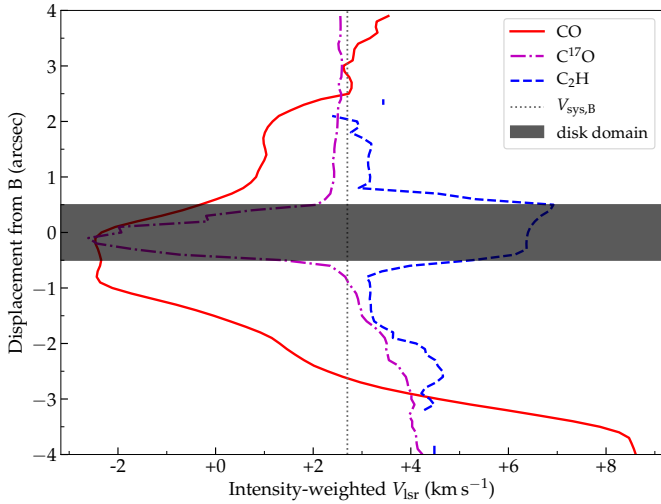
Fig. 7. Position-velocity diagram along the slice indicated by the arrow in Fig. 4. Velocity is the intensity-weighted peak velocity, as in Fig. 2. Position displacement is defined to be positive to the north of source B. The “disk domain”, inside which intensity-weighted velocity values are not meaningful, is marked with a partly transparent gray box.
