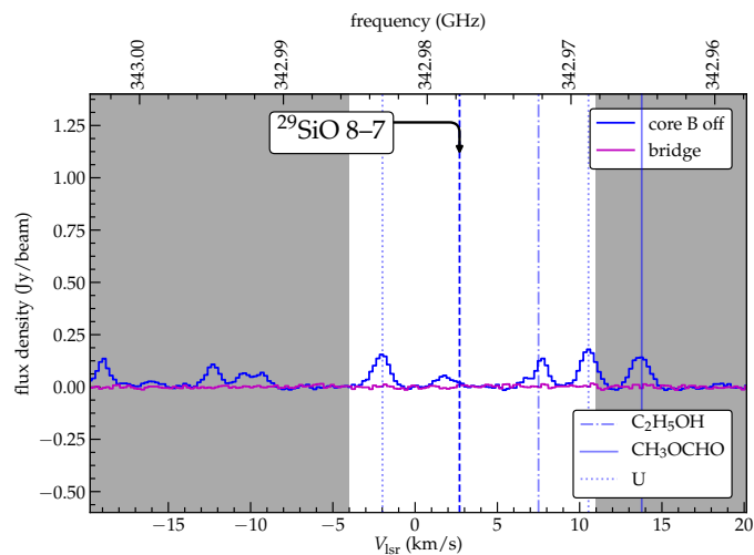
Fig. A.7. Same as Fig. A.1, but for 29 SiO.
