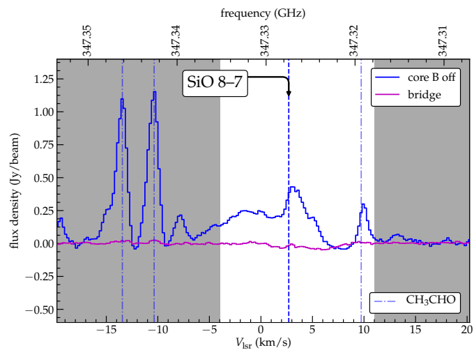
Fig. A.6. Same as Fig. A.1, but for SiO.
