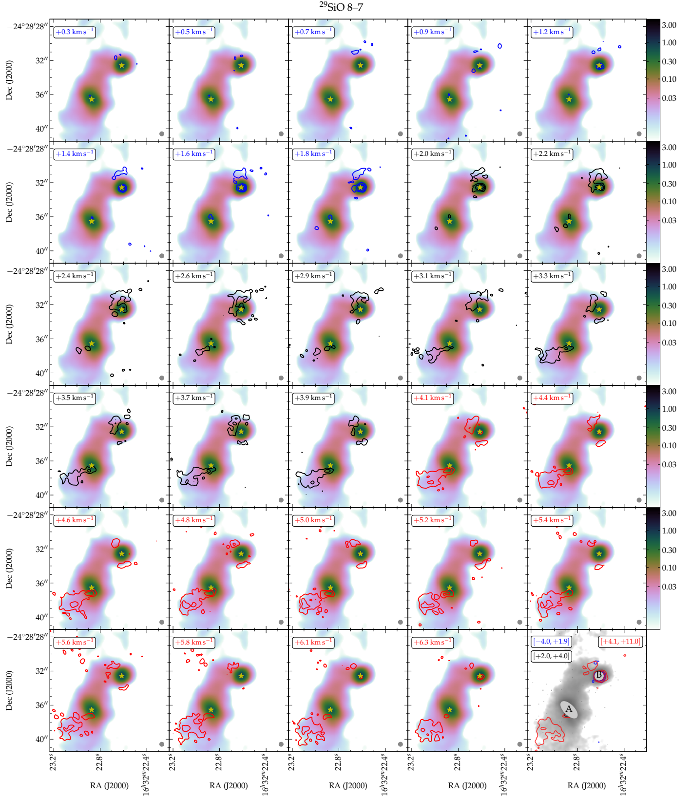
Fig. B.7. ^{29}\text{SiO} 8–7 channel maps. As Fig. B.1. First positive (negative) contour level in individual channel maps: 0.02 ( -0.04 ) \text{Jy beam}^{-1} ; first contour levels in the bottom right integrated ranges panel: 0.07 \text{Jy beam}^{-1} \text{ km s}^{-1} .
