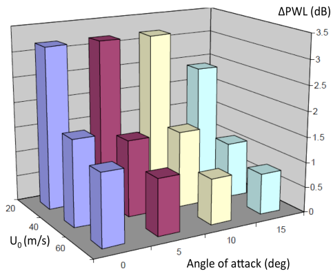
Figure 5. PWL reductions (dB) using 3S wing
