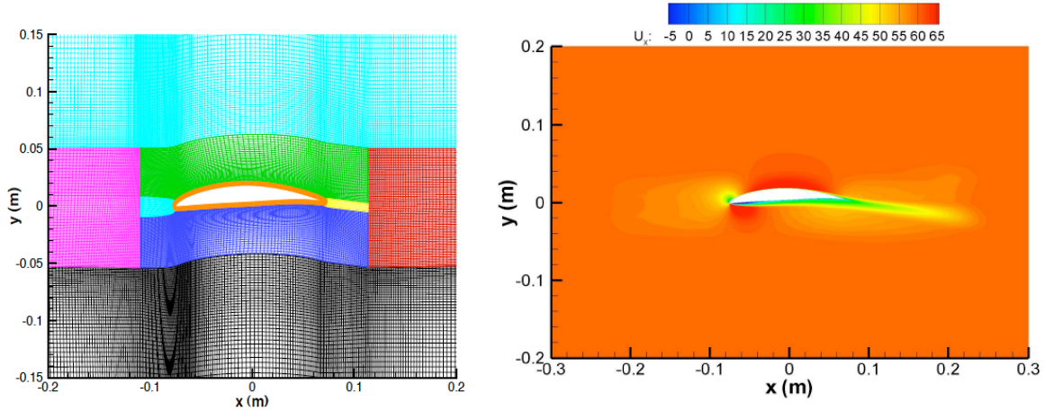
Figure 17. 2D CAA multi-bloc grid around airfoil (left) and RANS interpolated mean flow (right)
