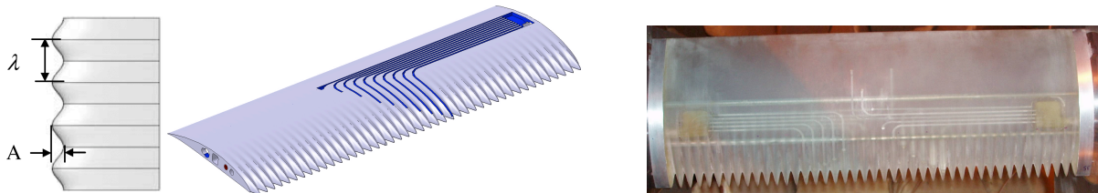
Figure 1. FLOCON wing design: CAD drawing (left) and manufactured wing (right)
