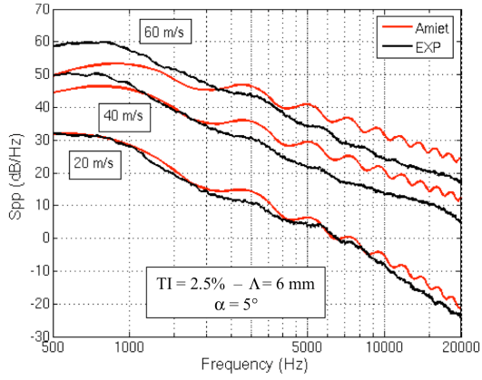
Figure 12. Predicted and measured PSD at 90°
