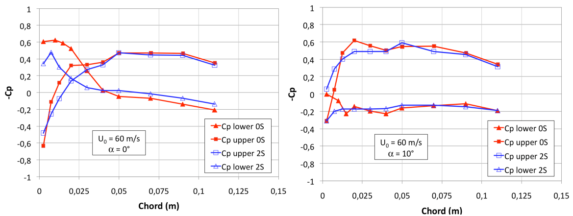
Figure 8. C_p distributions for baseline and ONERA 2S wing measured at \alpha = 0^\circ (left) and \alpha = 10^\circ (right)
