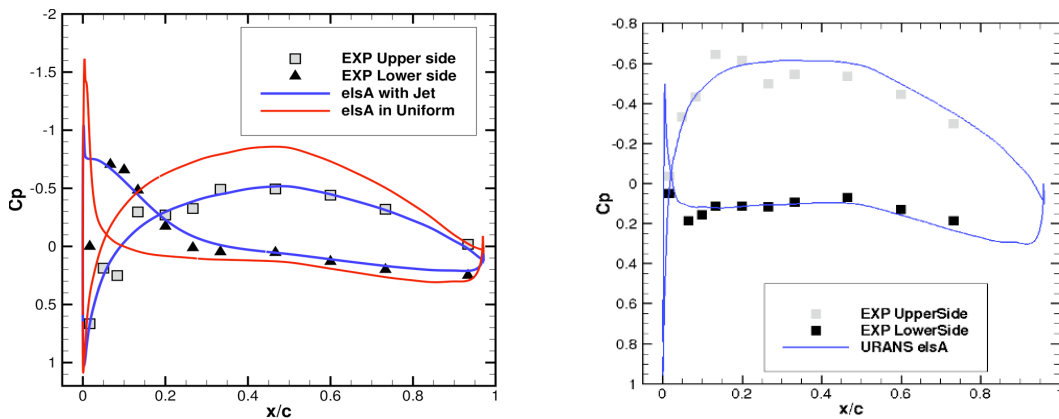
Figure 7. C_p distributions issued from RANS and measurements at \alpha = 0^\circ (left) and \alpha = 10^\circ (right)
