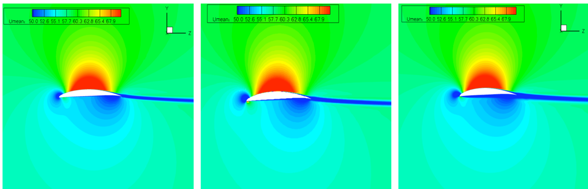
Figure 10. Spanwise cuts of RANS mean flow velocity field around 2S and baseline wings: 2S top wave (left), baseline (middle), and 2S bottom wave (right)
