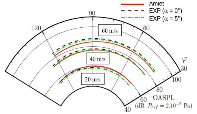
Figure 13. Predicted and measured OASPL directivities
