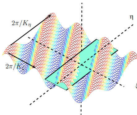
Figure 11. Sketch of gust-airfoil problem
