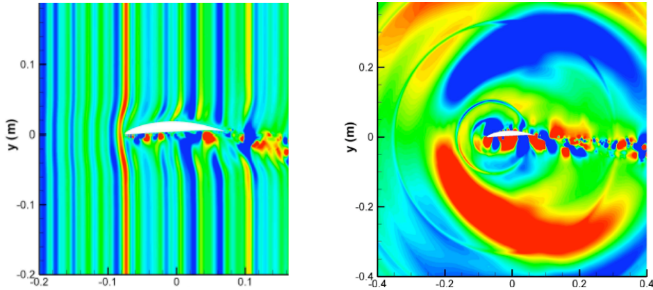
Figure 18. Synthetic turbulent velocity field (left) and direct acoustic pressure radiation (right)
