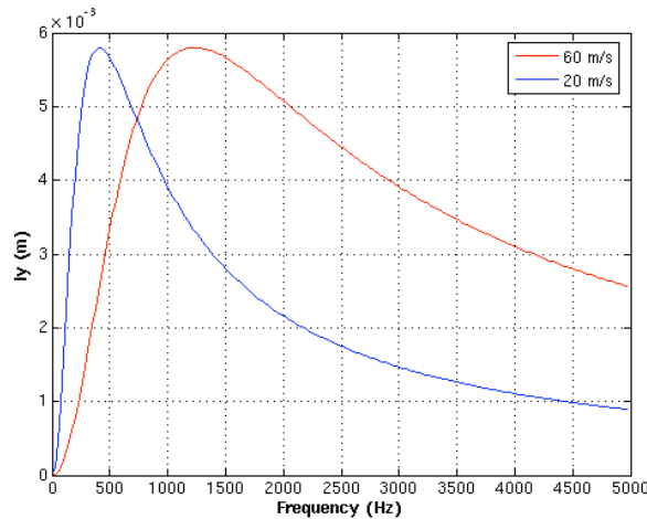
Figure 14. Spanwise correlation lengthscale deduced from ISVR turbulence grid characteristics
