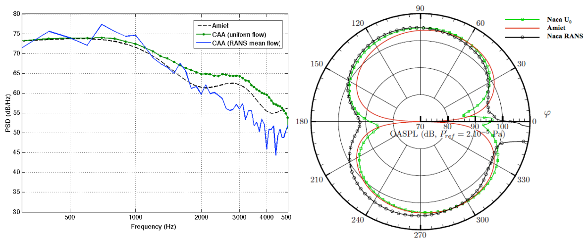
Figure 19. Predicted 2D spectra (dB/Hz) and OASPL (dB) directivities
