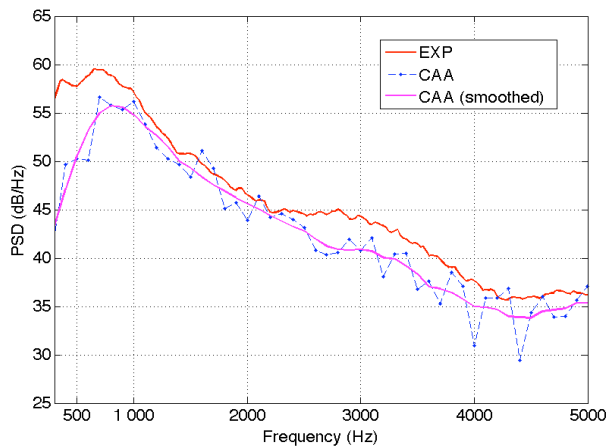
Figure 20. Predicted and measured 3D spectra (dB/Hz)
