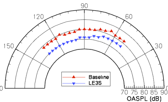
Figure 6. Baseline-3S comparisons of PWL (left) and OASPL directivities (right) at higher speed (60 m/s)
