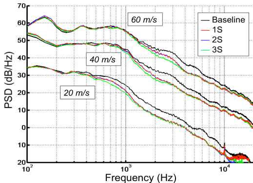
Figure 4. Baseline and ONERA wing spectra ( 90^\circ )
