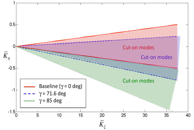
Figure 16. Spatial filtering of oblique gusts
