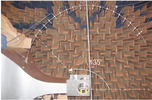
Figure 2. Experimental set-up in ISVR rig
