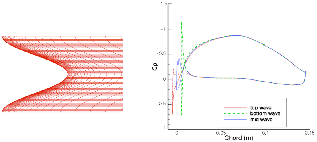
Figure 9. 3D RANS wavy-edge mesh (left) and computed C_p distributions ( U_0 = 60 \text{ m/s} , \alpha = 0^\circ )
