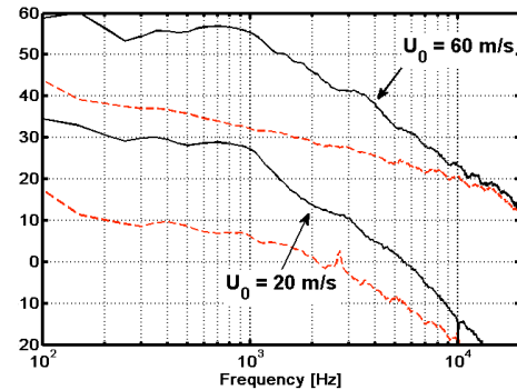
Figure 3. Interaction (black) and self (red) noise spectra
