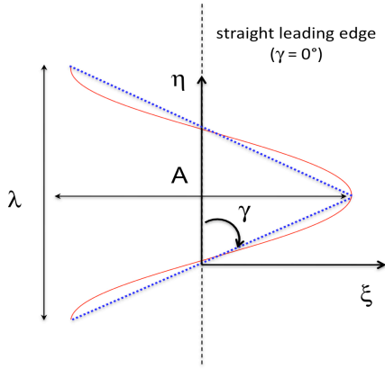
Figure 15. Sketch of triangular wave geometry
