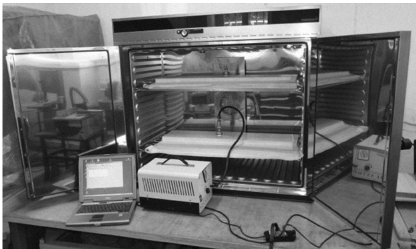
Fig.3 Sealed wood packages in a lab oven during the vacuum procedure.
