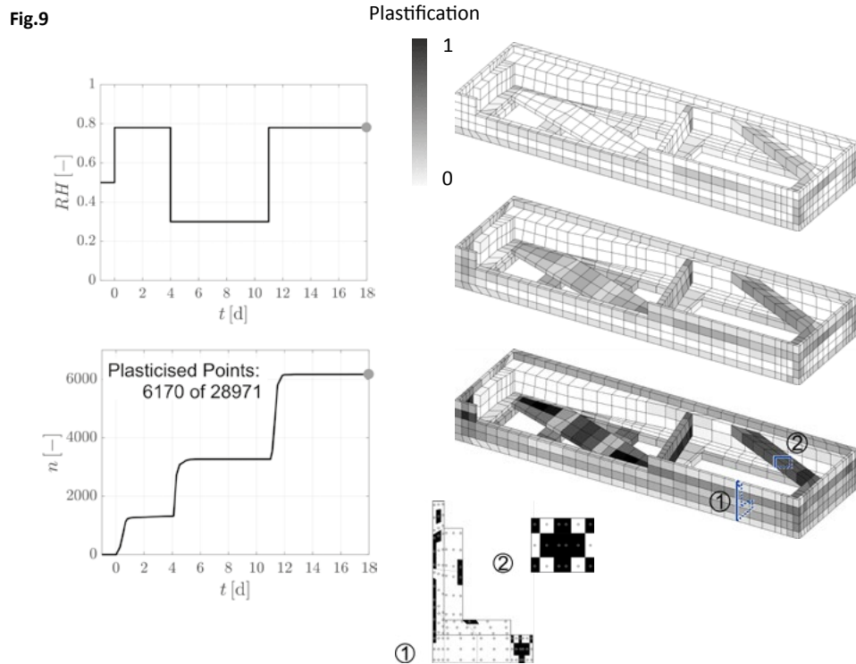
Fig.9 External climate loading RH(t) , number of plasticised integration points n(t) and degrees of plasticisation of the structures elements at the end of each cycle (from top to bottom) with the plasticised cross-sections of side wall ① and wrestplank ② after 18 days.
