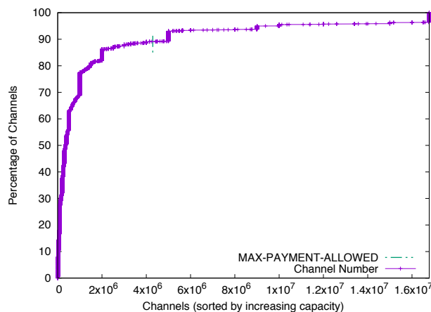
Figure 3. Percentage of deanonymizable channels, per number of channels attacked, sorted by increasing capacity.
