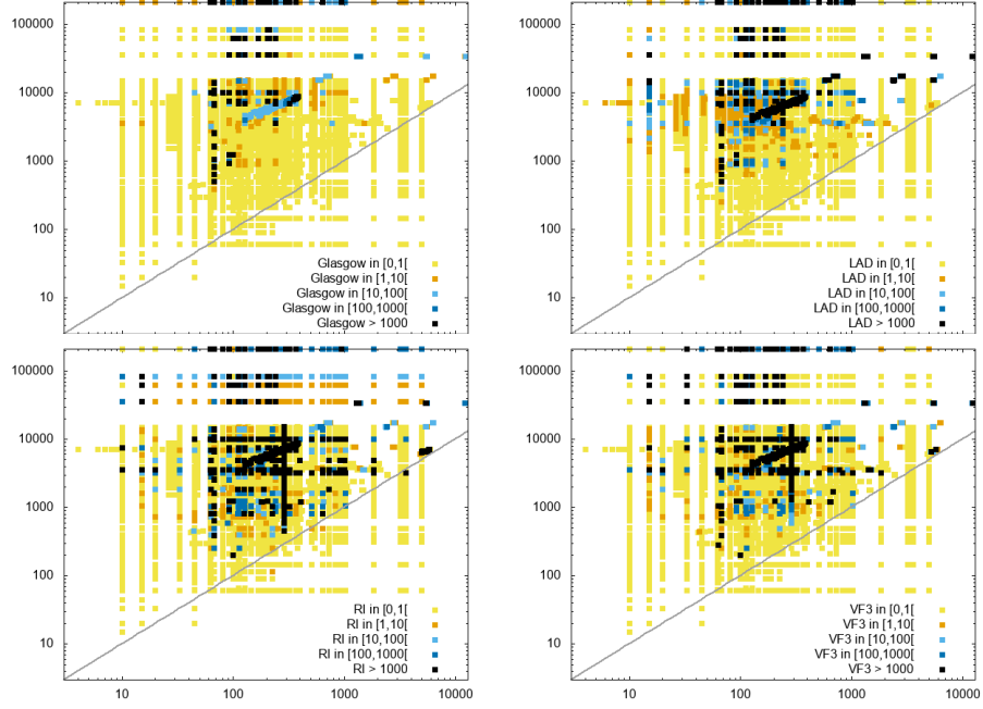
Fig. 2. Number of pattern edges (x-axis), target edges (y-axis), and solving time (colour) for induced SI: top left = Glasgow; top right = LAD; bottom left = RI; bottom right = VF3.
