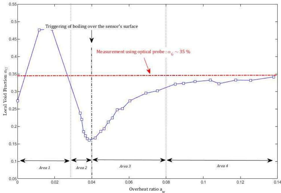
Figure 15. Influence of the overheat ratio on the void fraction determination using anemometry. Boiling occurs for \alpha_w = 0.04
