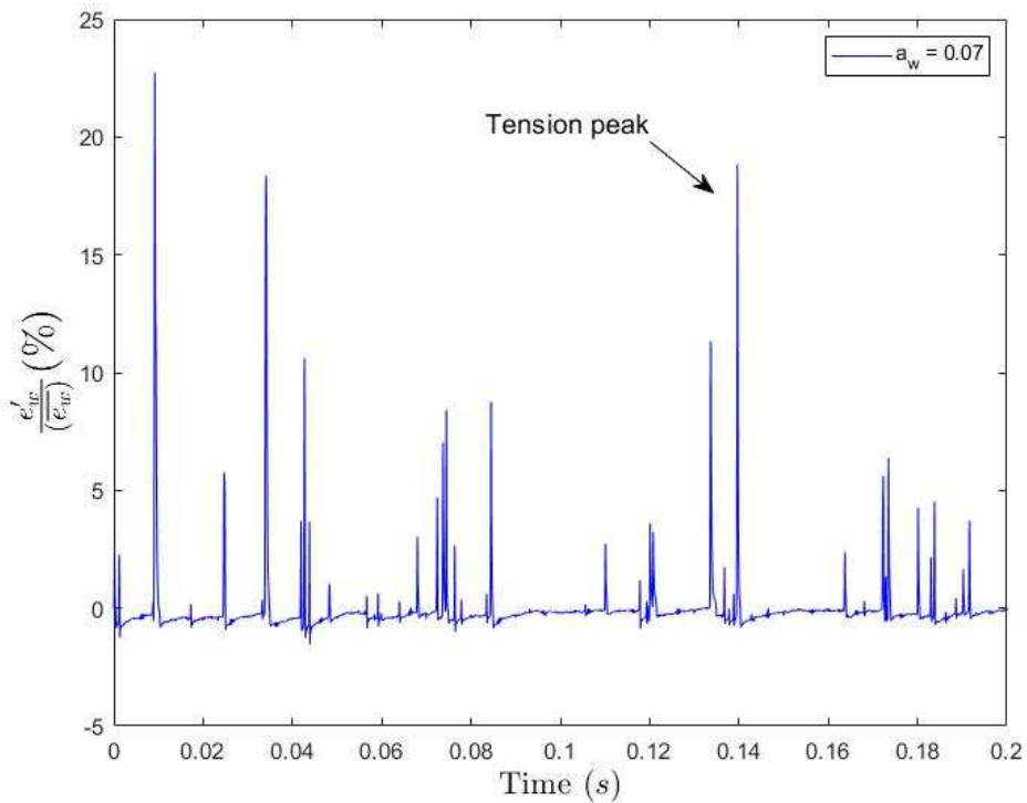
Figure 11: Fluctuations of the normalized voltage of the sensor ( e'_w/\overline{e_w} ) a_w = 0.07 . Boiling occurs at a_w \geq 0.04 . Void fraction \alpha = 4\%
