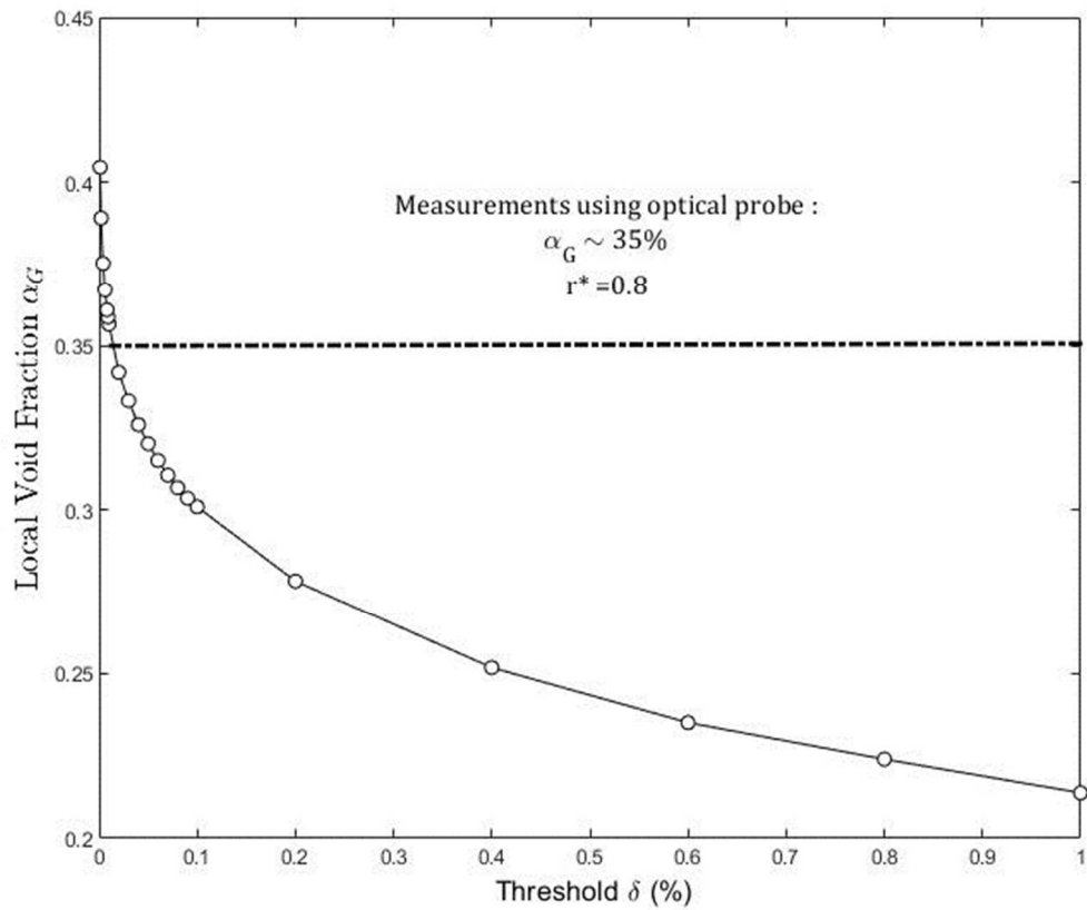
Figure 13: the best value of \delta is determined for void fraction measured at r^* = r/R = 0.8 . Measurements have been performed with a Tungsten wire probe d = 5 \mu m
