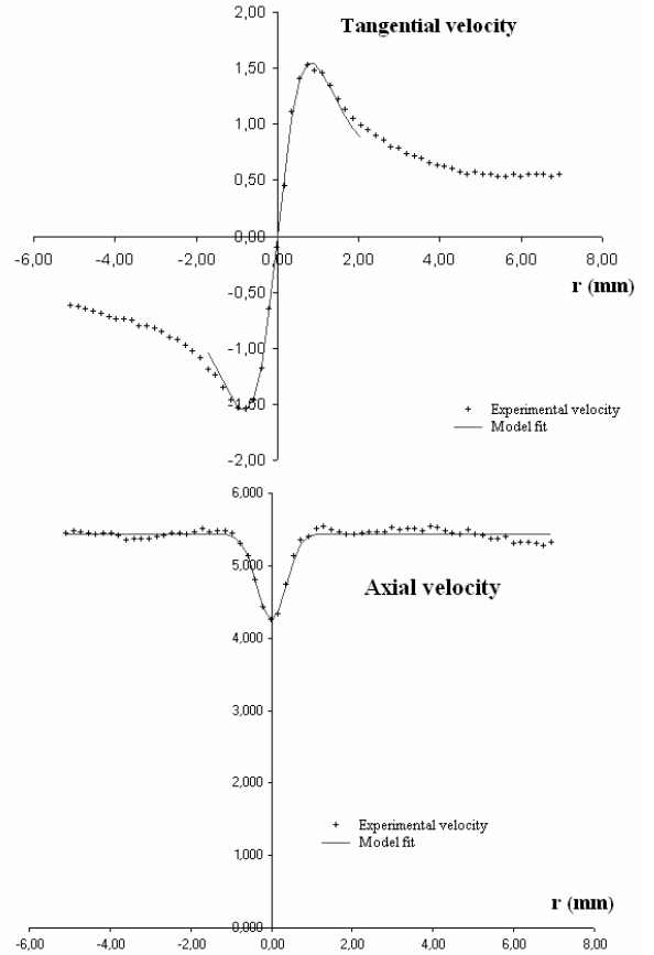
Figure 5: Example of tangential and axial velocity fit
