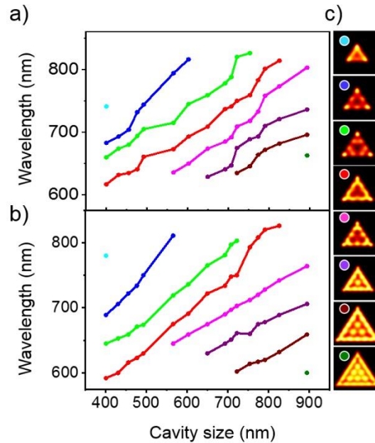
Figure 3: (a-b) High order SP resonance dispersion. The spectral position of the fitted (a) and computed (b) resonances is plotted as a function of the cavity edge size. A similar color code is used in Figure 2 and 3. (c) SP-LDOS maps corresponding to the resonances with the same color code.
