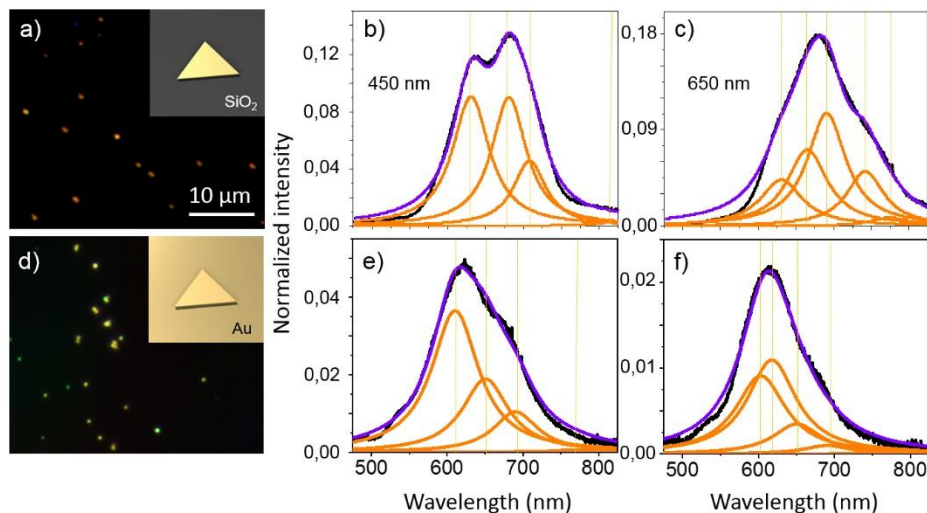
Figure 4: (a) and (d) show dark field images of Au cavities on ITO-covered glass and Au thin film respectively. Artistic views of the two configurations are shown in inset. DF spectra
