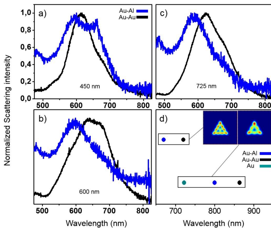
Figure 7: (a-c) Normalized DF scattering spectra of gold nanoprism of sizes (a) 450 nm, (b) 600 nm and (c) 725 nm on two different metallic substrates – 30 nm thick gold film (black) and 30 nm thick aluminum film (blue). (d) Spectral position of two resonances as a function of the substrate nature (blue: aluminum; black: gold; cyan: ITO/glass). The spatial distributions corresponding to the two resonances are shown in inset.
