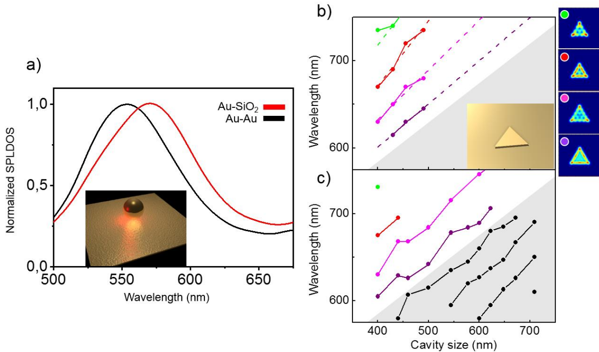
Figure 5: (a) Simulated SP-LDOS spectra of a 60 nm Au nanosphere positioned 10 nm above a 45 nm thick gold film. (b-c) High order SP resonance dispersion. The spectral position of the computed (a) and fitted (b) resonances is plotted as a function of the cavity edge size. A similar color code is used in Figure 2 and 3. SP-LDOS maps corresponding to the resonances with the same color code (colored dots).
