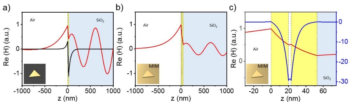
Figure 6: (a) Simulated profiles of the real part of the magnetic field associated to the plasmon bound to the upper air-Au (red curve) and lower Au-glass (black curve) interfaces at \lambda=600 nm on a 400 nm wide prism. (b) Similar as (a) for the upper plasmon in the MIM configuration. The growing oscillations of the field signal that the mode, computed by solving the dispersion relation for the structure, is leaking in the substrate. (c) Profiles of the real part of the magnetic field of the upper plasmon and longitudinal gap plasmon in the MIM configuration.
